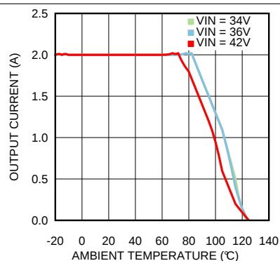
Figure 28. Thermal Derating V_{OUT} = 24\text{ V} , R_{\theta JA} = 20^\circ\text{C/W}
