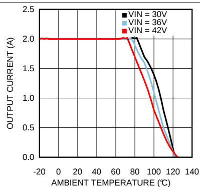
Figure 26. Thermal Derating V_{OUT} = 12\text{ V} , R_{\theta JA} = 20^\circ\text{C/W}
