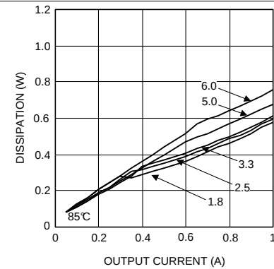
Figure 16. Dissipation 12-V Input at 85°C
