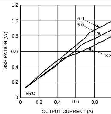
Figure 20. Dissipation 36-V Input at 85°C
