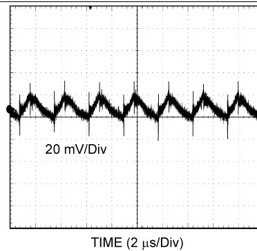
Figure 34. Output Ripple
