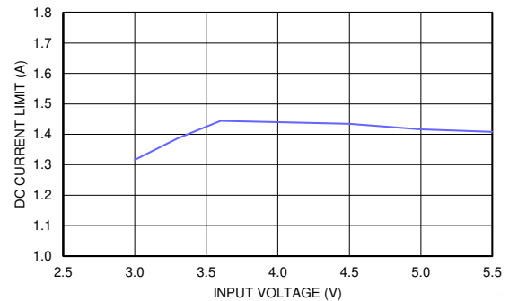
Figure 8-19. DC Current Limit V_{OUT} = 2.5\text{ V} , T_A = 85^\circ\text{C}
