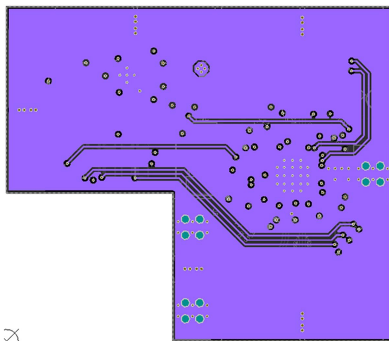
Figure 98. Mid Layer 3
