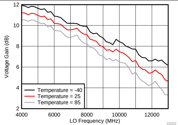
Figure 4. Voltage Gain Across LO frequency for External LO Mode
