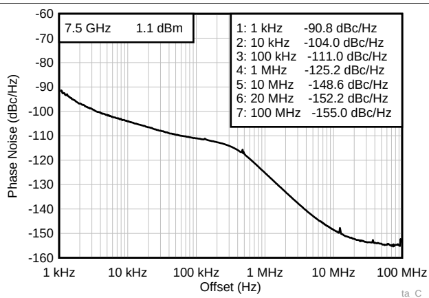
Figure 93. Direct VCO Noise
