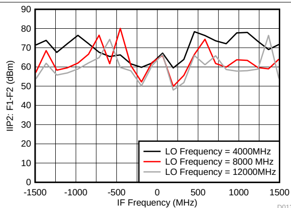
Figure 12. IIP2: F1-F2 Across LO Frequency for External LO Mode
