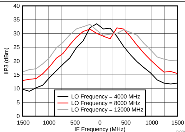
Figure 10. IIP3 Across IF Frequency for External LO Mode
