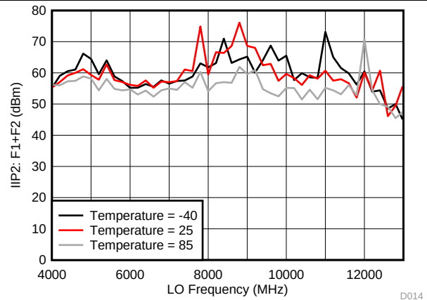
Figure 16. IIP2: F1+F2 Across LO Frequency for External LO Mode
