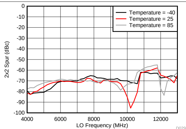
Figure 32. 2x2 Spur for Internal LO Mode
