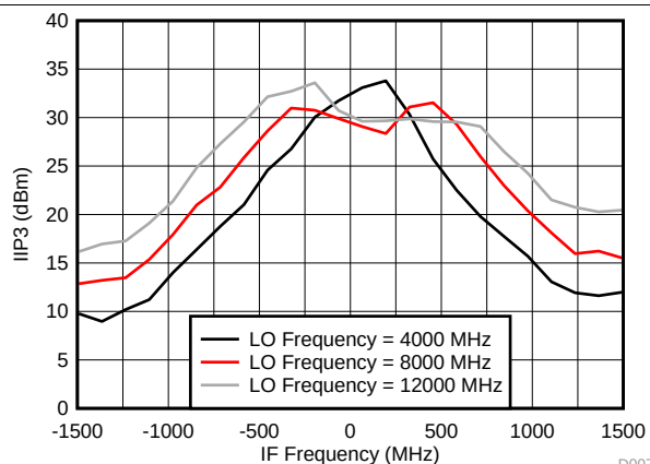
Figure 9. IIP3 Across IF Frequency for Internal LO Mode
