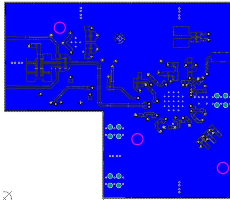
Figure 99. Bottom Layer
