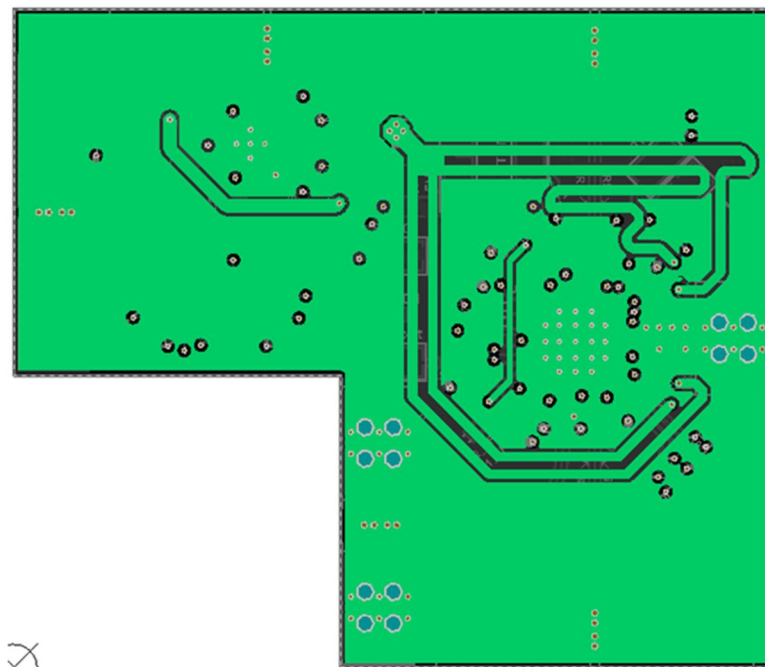
Figure 97. Mid Layer 2
