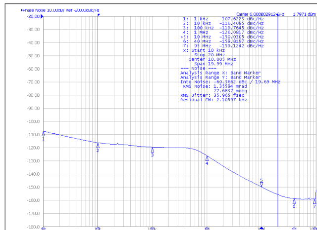
Figure 8-2. Measurement Plot
