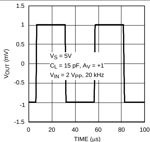
Figure 30. Large Signal Transient Response
