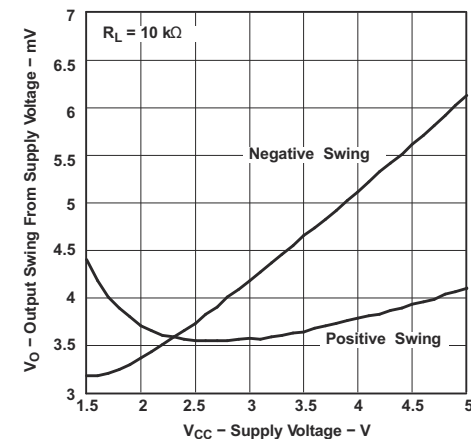
Figure 5-4. Output Voltage Swing vs Supply Voltage
