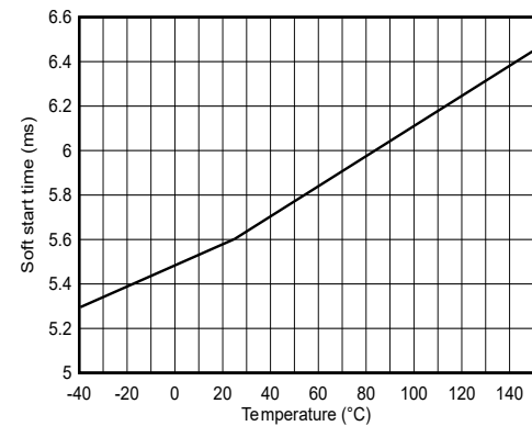
Figure 6-6. Soft Start Time
