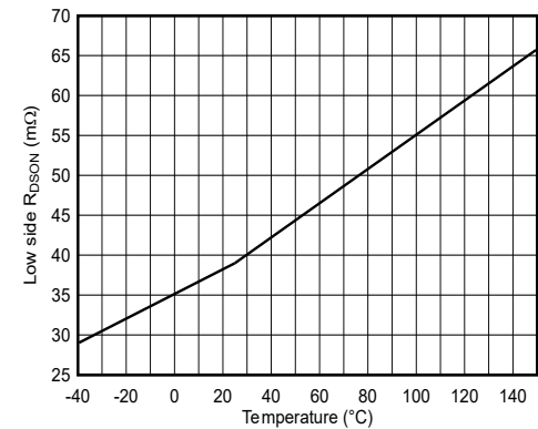
Figure 6-4. Low Side MOSFET R_{DS-ON}
