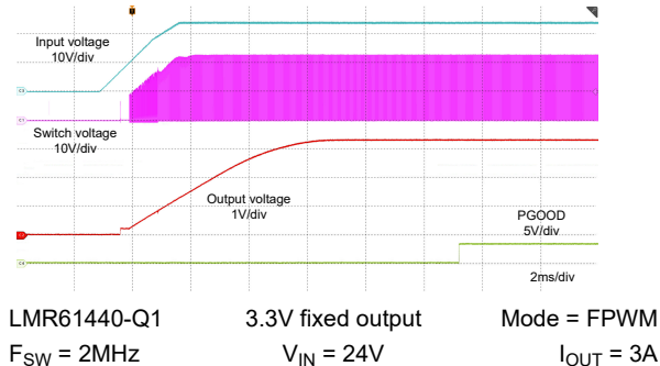
Figure 8-8. Start-Up Operation
