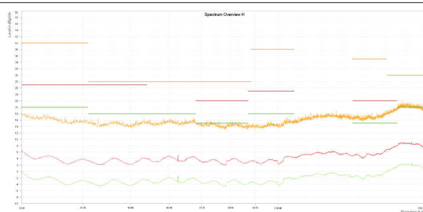
Figure 8-26. Radiated EMI Monopole versus CISPR25 Limits, LMR60440QEV
