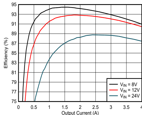
Figure 8-5. Efficiency
