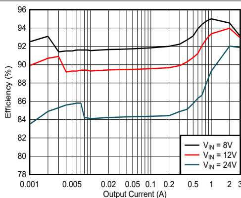
Figure 8-2. Efficiency
