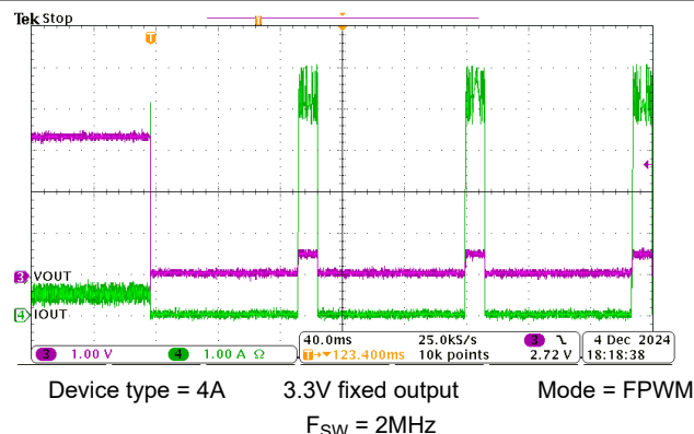
Figure 8-21. Short-Circuit Applied
