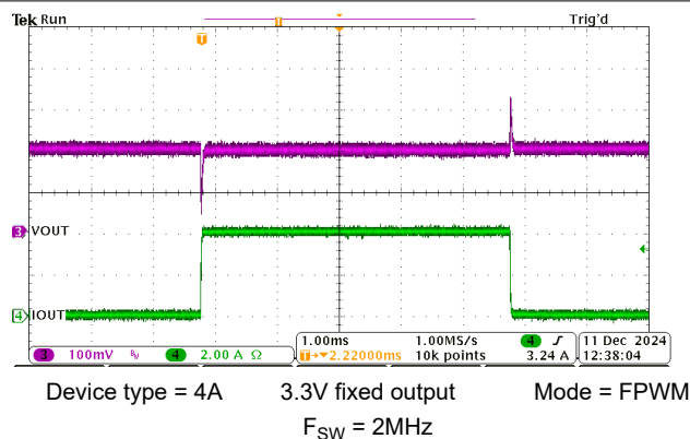
Figure 8-17. 20mA to 4A Load Transient
