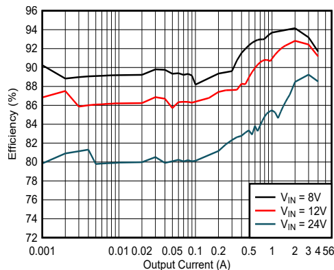
Figure 8-4. Efficiency
