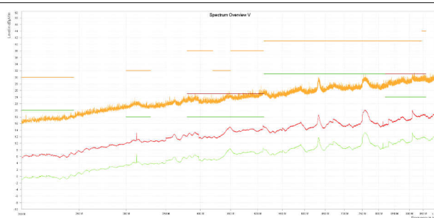
Figure 8-27. Radiated EMI Bicon Vertical versus CISPR25 Limits, LMR60440QEV
