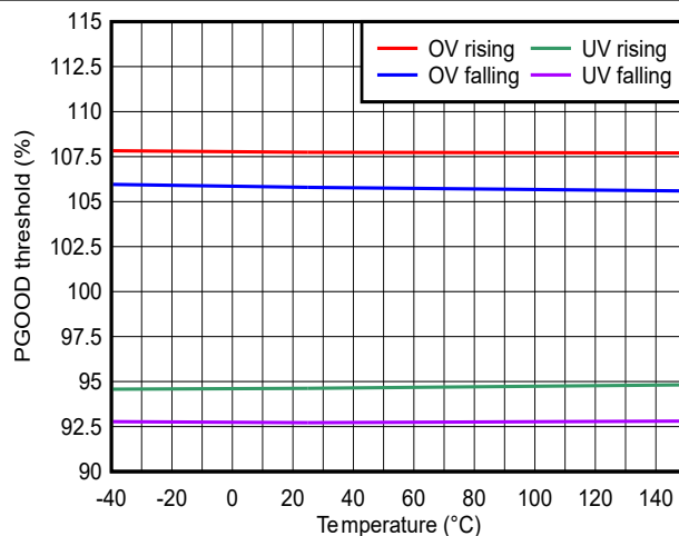
Figure 6-10. PGOOD Thresholds
