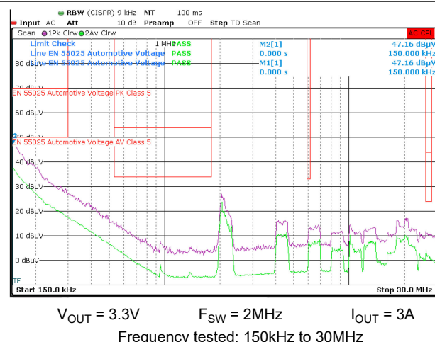
Figure 8-24. Conducted EMI versus CISPR25 Limits (Purple: Peak Signal, Green: Average Signal), LMR60440QEV
