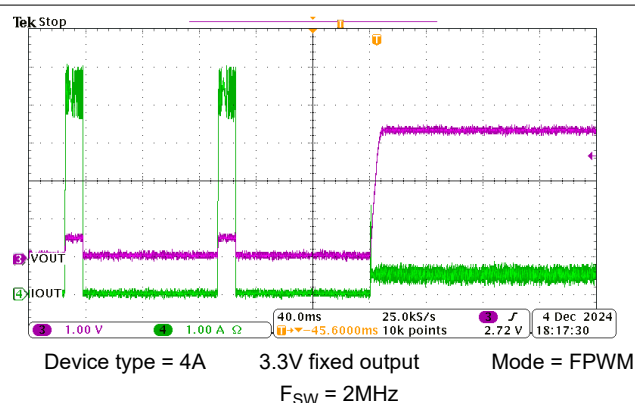
Figure 8-22. Short-Circuit Recovery
