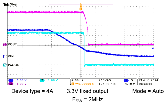
Figure 8-20. Shutdown Operation
