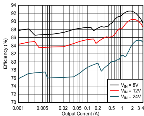
Figure 8-2. Efficiency
