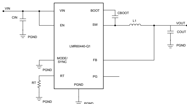
Simplified Schematic – Fixed Output
