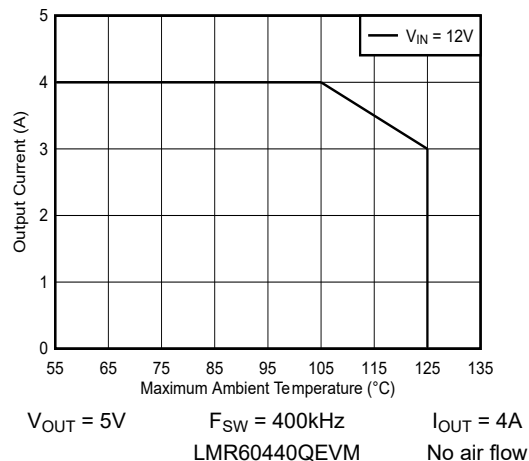
Figure 8-15. Output Current vs Maximum Ambient Temperature
