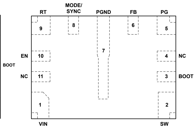
Figure 5-2. RBM Package 11-Pin WQFN-HR (Top View)
