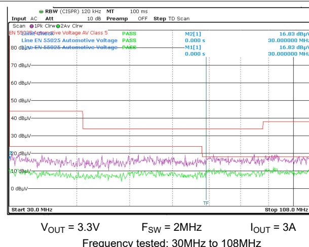
Figure 8-25. Conducted EMI versus CISPR25 Limits (Purple: Peak Signal, Green: Average Signal), LMR60440QEV
