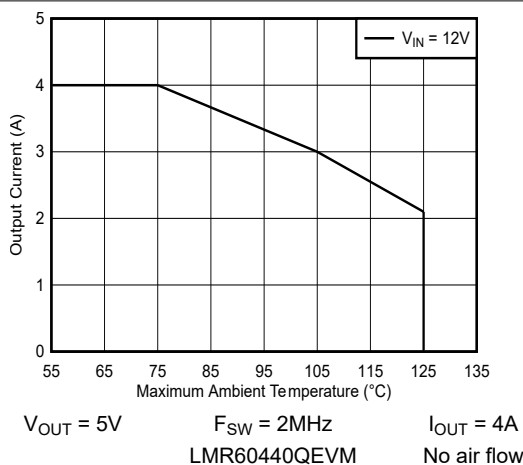
Figure 8-16. Output Current vs Maximum Ambient Temperature
