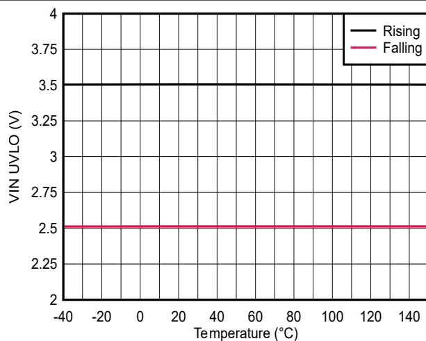
Figure 6-9. Input Voltage UVLO
