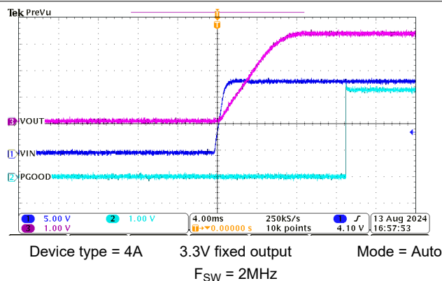
Figure 8-19. Start-Up Operation
