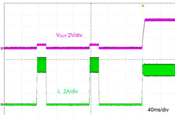
Figure 8-9. Short Recovery
