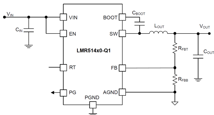
Simplified Schematic
