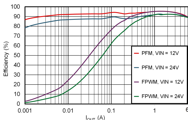
Efficiency vs Output Current V_{\text{OUT}} = 5\text{V} , 400kHz
