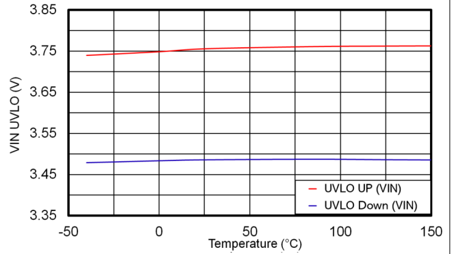
Figure 6-8. V_{IN} UVLO
