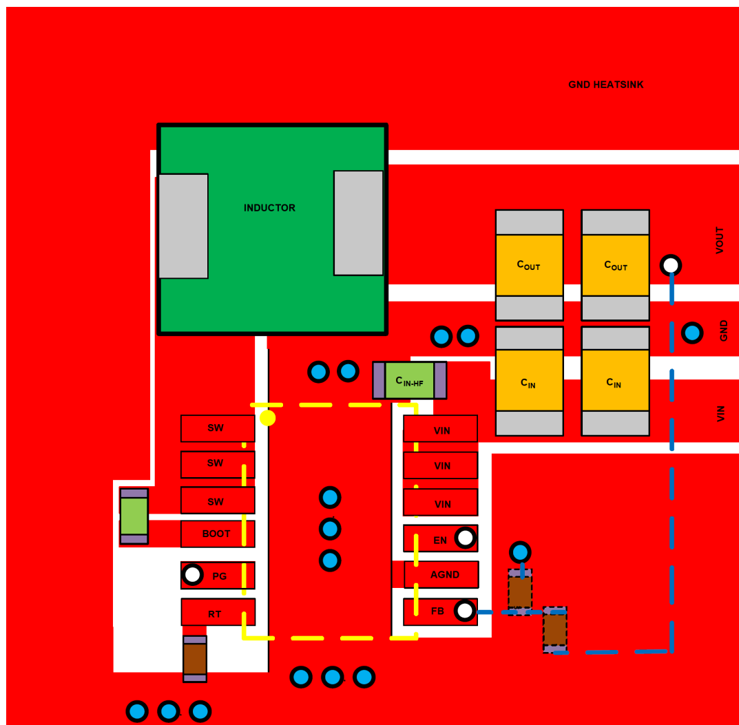
Figure 8-10. Layout
