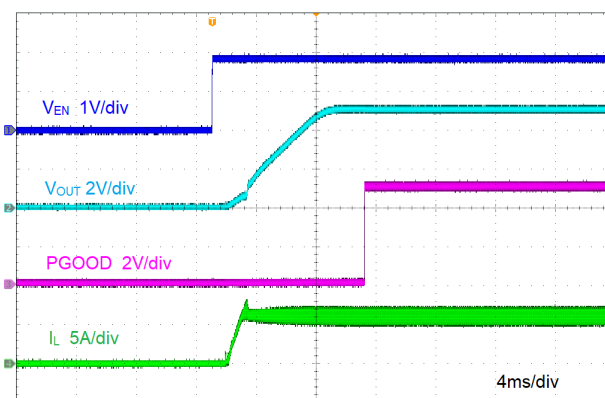
Figure 8-5. Start-Up by EN
