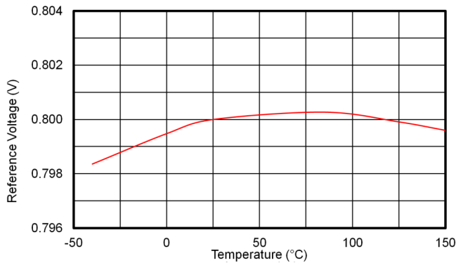
Figure 6-9. Reference Voltage
