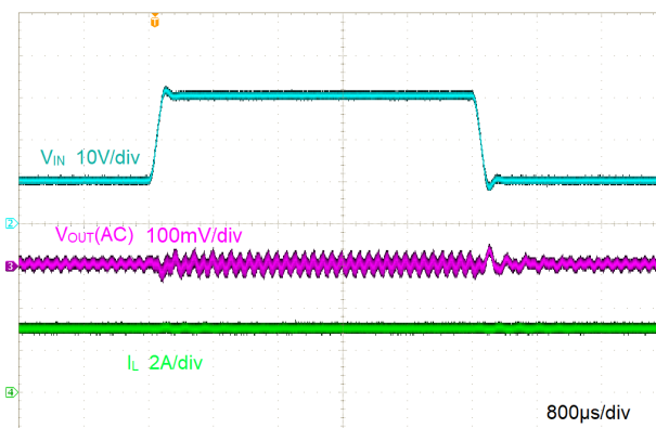
Figure 8-7. Line Transient
