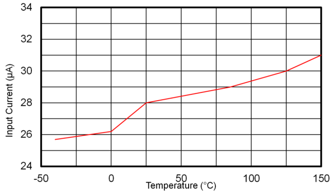
Figure 6-7. Non-Switching Input Supply Current
