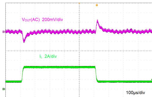
Figure 8-6. Load Transient
