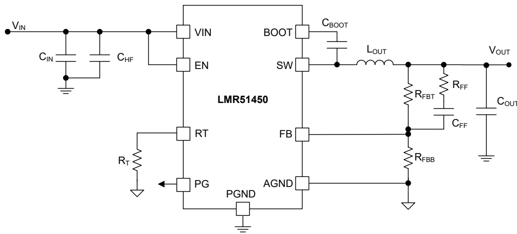
Figure 9-1. Application Circuit
