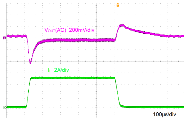
Figure 9-6. Load Transient
