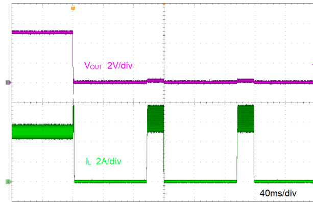
Figure 9-8. Short Protection
