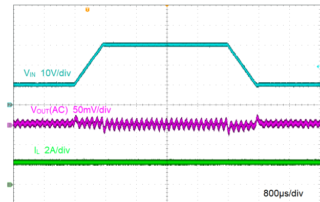
Figure 9-7. Line Transient
