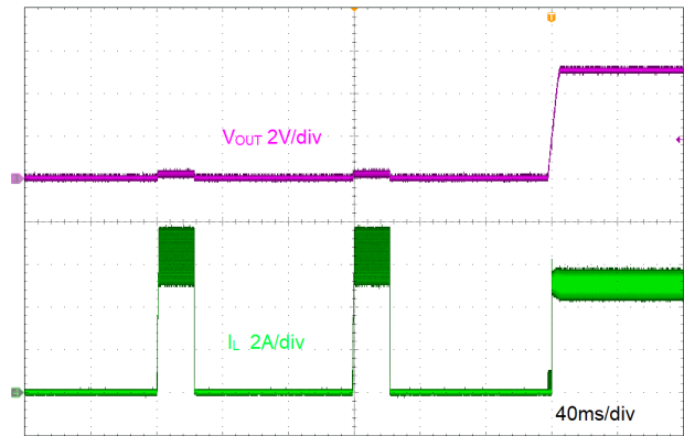
Figure 9-9. Short Recovery
