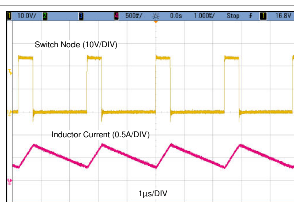
Figure 7-8. Typical PWM Switching Waveforms V_{IN} = 24\text{ V} , V_{OUT} = 5\text{ V} , I_{OUT} = 0.5\text{ A} , f_S = 400\text{ kHz}
