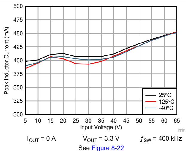
Figure 6-2. I_{PEAK-MIN}
