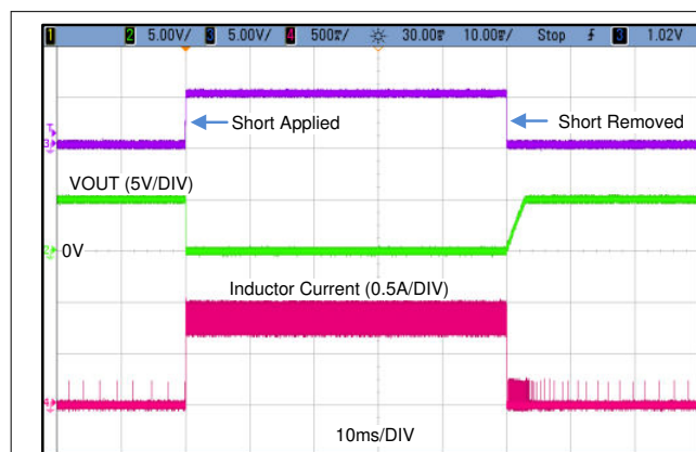
Figure 7-12. Short-Circuit Waveform
