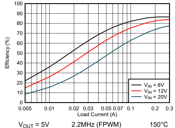
Figure 8-11. Efficiency
