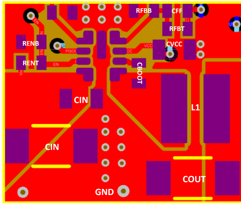
Figure 8-34. Example Layout
