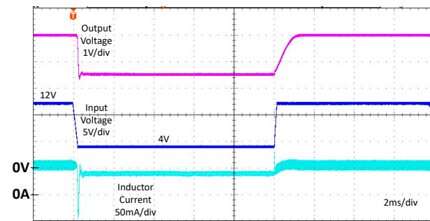
Figure 7-9. Dropout Performance: I_{OUT} = 50\text{ mA}
