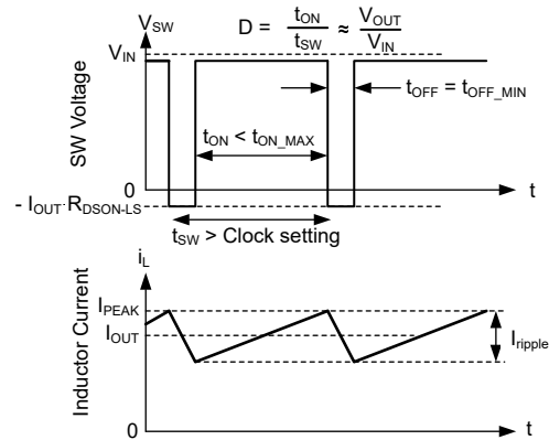
Figure 7-19. Dropout Waveforms
