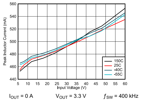
Figure 8-6. I_{PEAK-MIN}
