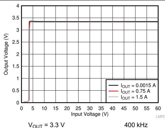
Figure 10-9. Line Regulation
