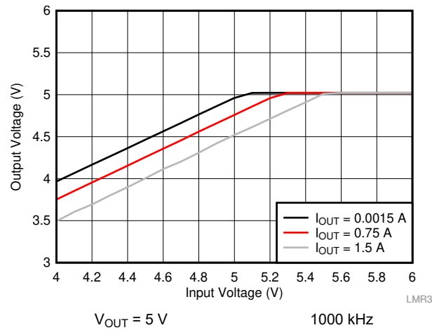
Figure 10-30. Overall Dropout Characteristic
