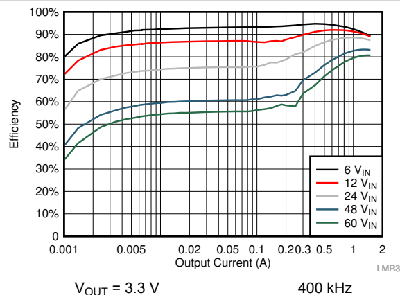
Figure 10-5. Efficiency
