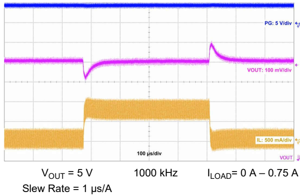
Figure 10-34. Load Transient
