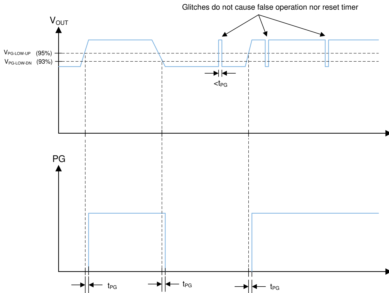
Figure 9-3. Power-Good-Timing Behavior
