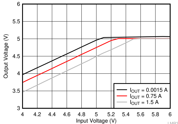
Figure 9-9. Overall Dropout Characteristic V OUT = 5 V
