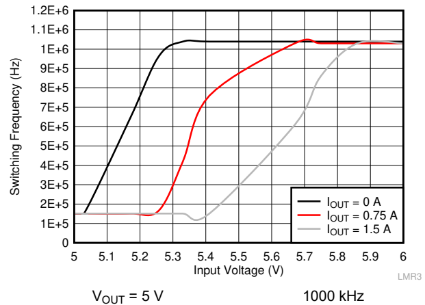
Figure 10-31. Frequency Dropout Characteristic
