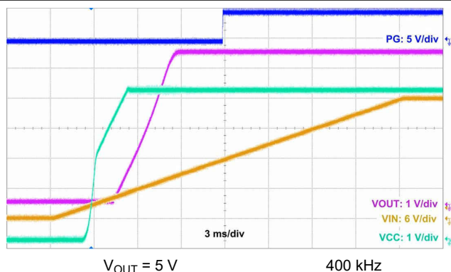
Figure 10-14. Start-Up Waveform
