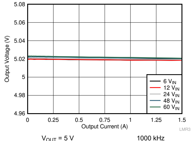
Figure 10-29. Load Regulation
