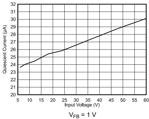
Figure 8-1. Non-Switching Input Supply Current
