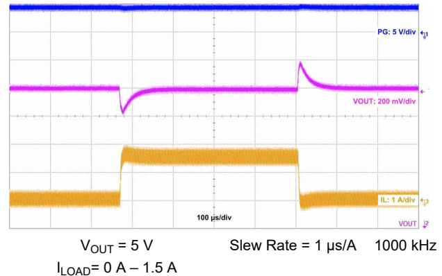
Figure 10-35. Load Transient
