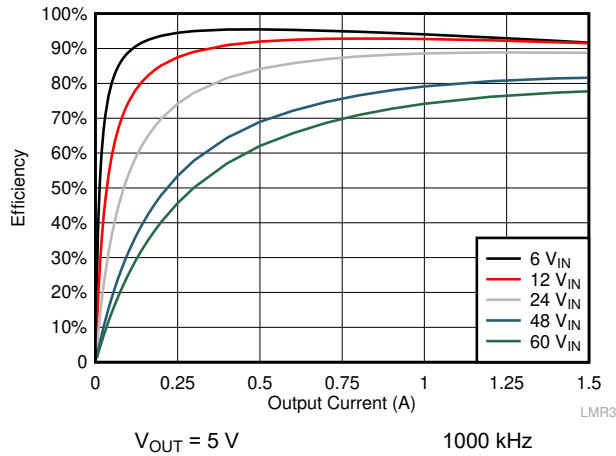
Figure 10-28. Efficiency
