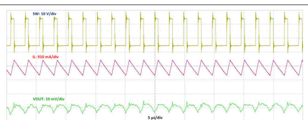
Figure 9-8. Typical PWM Switching Waveforms V_{IN} = 24\text{ V} , V_{OUT} = 5\text{ V} , I_{OUT} = 1.5\text{ A} , f_s = 400\text{ kHz}
