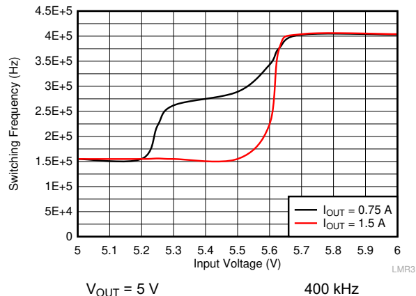
Figure 10-11. Frequency Dropout Characteristic
