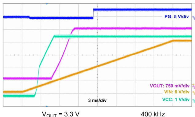
Figure 10-15. Start-Up Waveform
