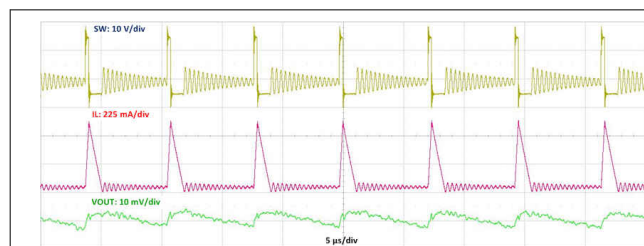
Figure 9-7. Typical PFM Switching Waveforms V_{IN} = 24\text{ V} , V_{OUT} = 5\text{ V} , I_{OUT} = 200\text{ mA}
