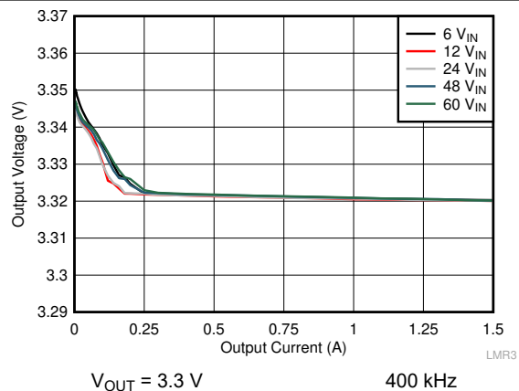
Figure 10-7. Load Regulation
