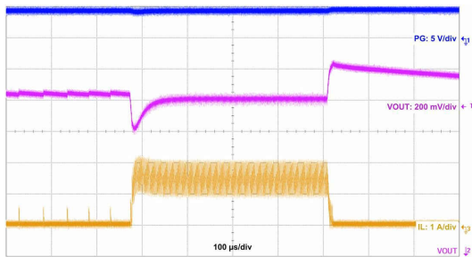
Figure 10-16. Load Transient
