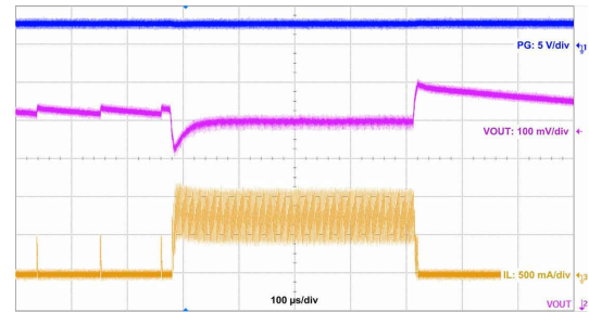
Figure 10-17. Load Transient
