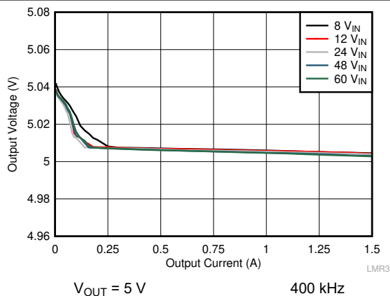
Figure 10-6. Load Regulation
