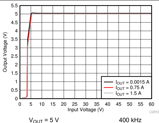
Figure 10-8. Line Regulation
