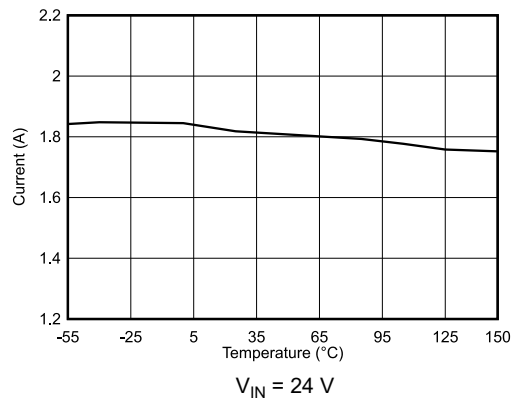
Figure 8-4. Low Side Current Limit
