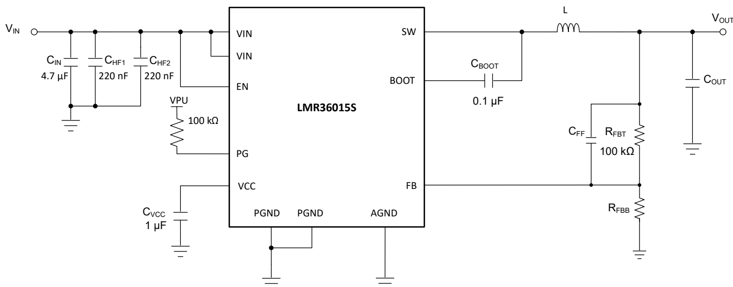
Figure 10-1. Example Applications Circuit
