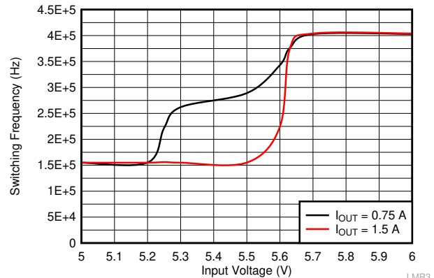
Figure 9-10. Frequency Dropout Characteristics f sw = 400 kHz
