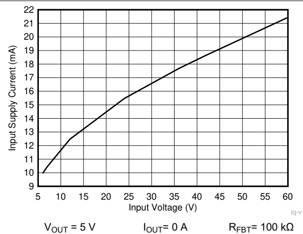
Figure 10-32. Input Supply Current
