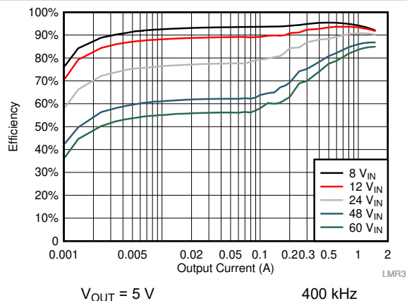
Figure 10-4. Efficiency
