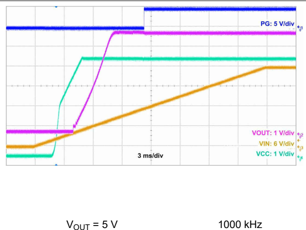
Figure 10-33. Start-Up Waveform
