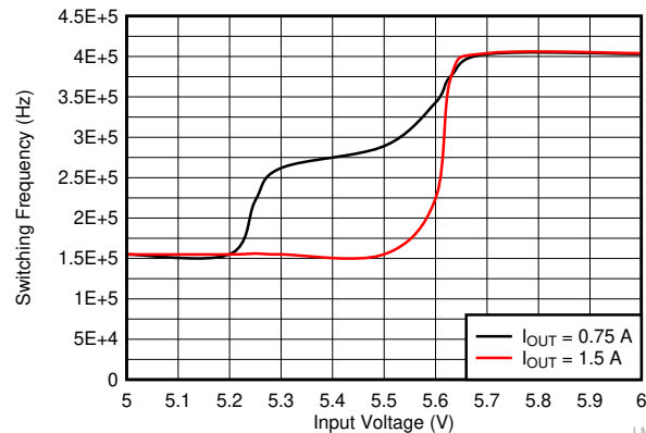
Figure 9-10. Frequency Dropout Characteristics f_{SW} = 400 kHz
