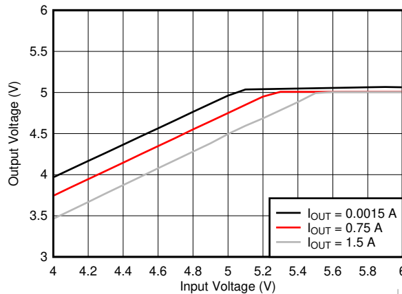
Figure 9-9. Overall Dropout Characteristic V_{OUT} = 5 V
