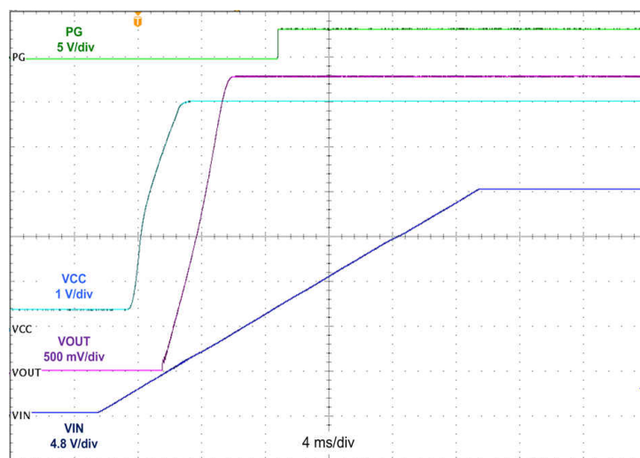
Figure 9-5. Typical Start-up Behavior V_{IN} = 24 V, V_{OUT} = 3.3 V, I_{OUT} = 1.5 A
