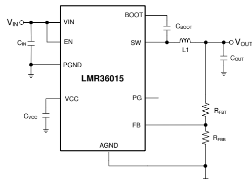
Simplified Schematic
