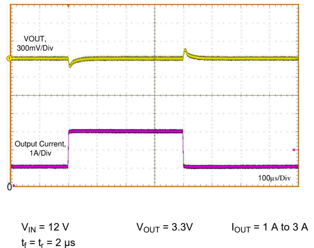
Figure 9-30. Load Transient
