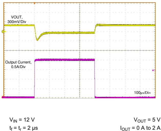
Figure 9-23. Load Transient
