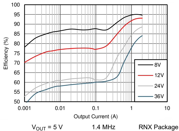
Figure 9-15. Efficiency
