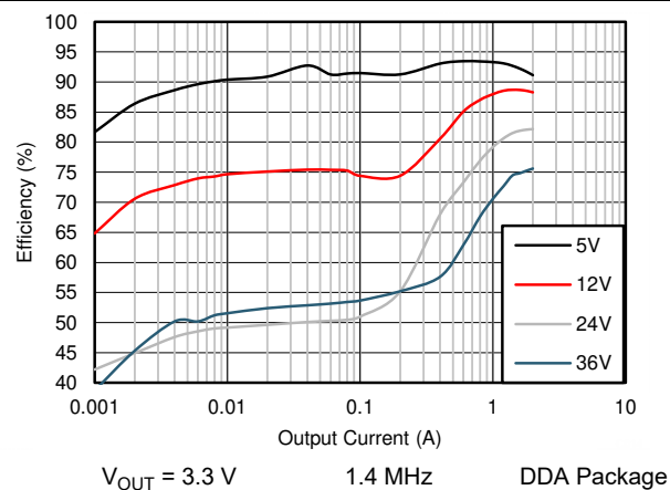
Figure 9-10. Efficiency
