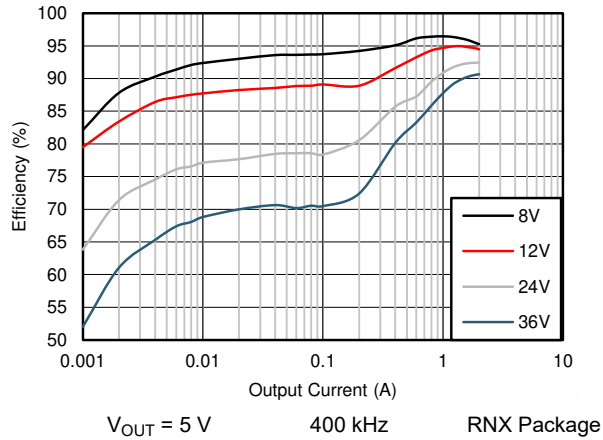
Figure 9-13. Efficiency
