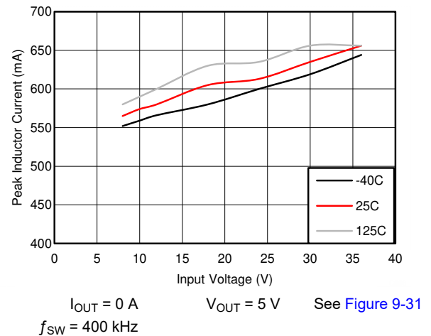
Figure 7-6. I_{PEAK-MIN}
