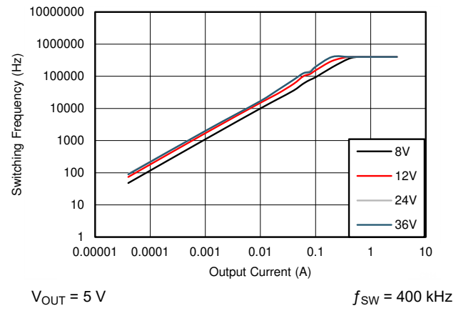
Figure 9-22. Switching Frequency versus Output Current
