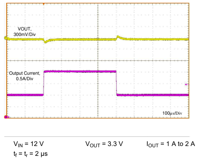
Figure 9-30. Load Transient
