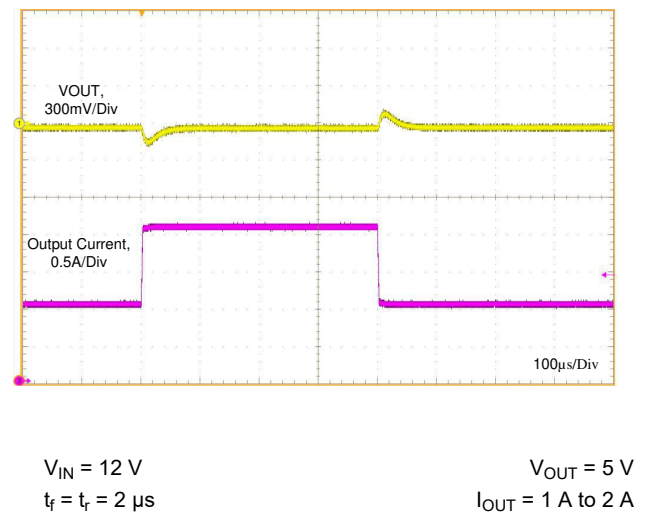
Figure 9-24. Load Transient
