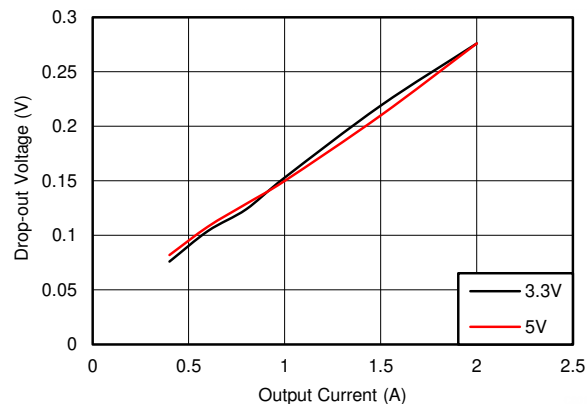
Figure 8-10. Typical Dropout Voltage versus Output Current in Frequency Foldback f_{SW} = 140 kHz
