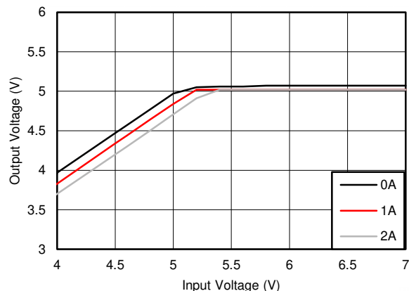
Figure 8-9. Overall Dropout Characteristic V_{OUT} = 5 V
