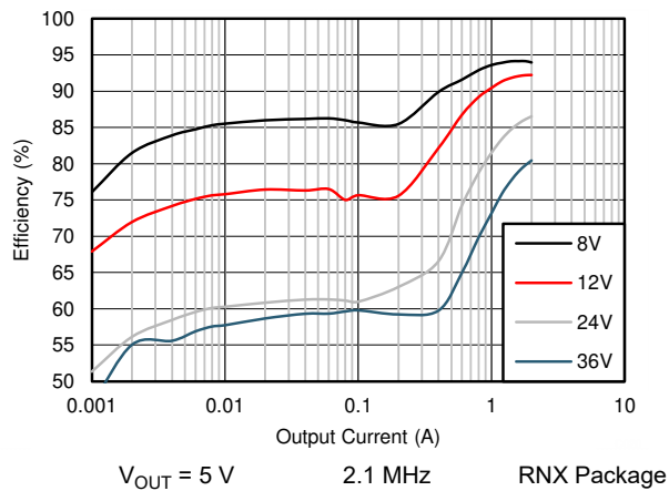
Figure 9-17. Efficiency
