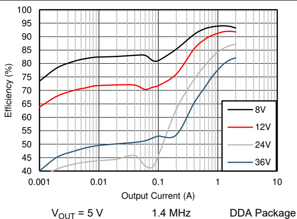
Figure 9-9. Efficiency
