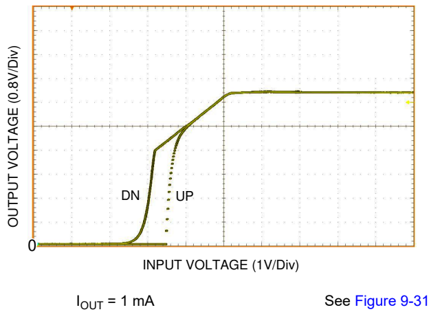
Figure 7-5. UVLO Thresholds
