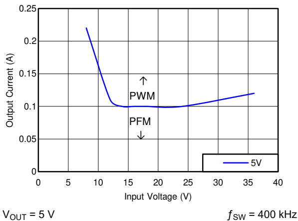
Figure 9-21. Mode Change Thresholds
