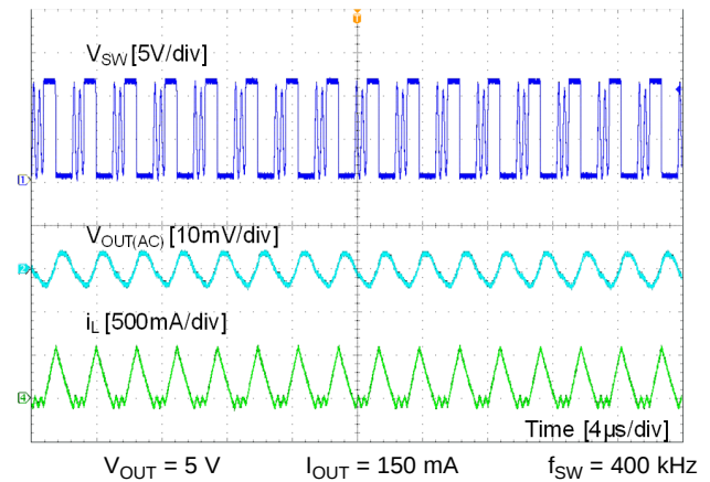
Figure 25. DCM Mode
