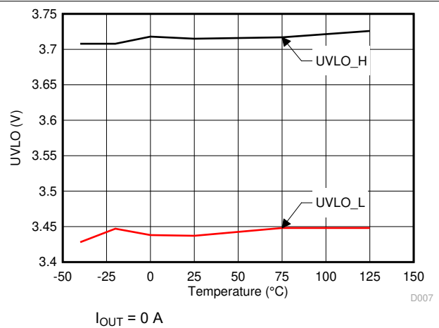
Figure 5-12. UVLO Threshold
