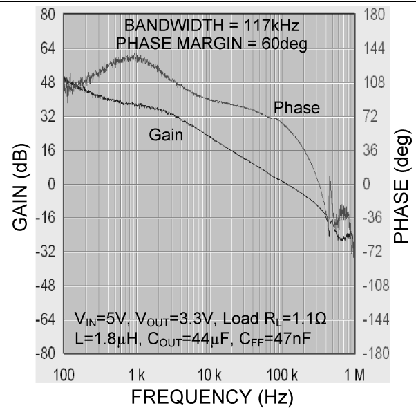
Figure 23. Loop Gain and Phase With C_{FF}
