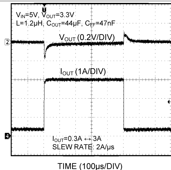
Figure 25. Load Step Response With C_{FF}
