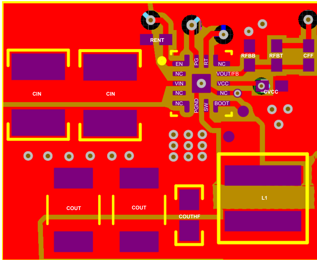
Figure 8-34. Example Layout
