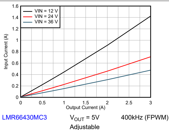
Figure 8-29. Input Current vs Load Current
