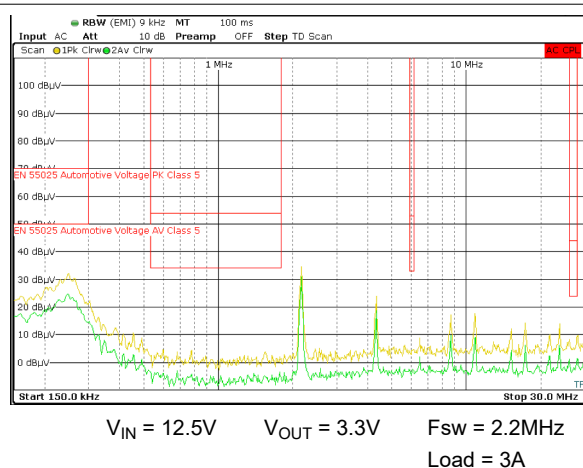
Figure 8-18. CISPR 25 Class 5 Conducted EMI 150 kHz–30MHz Yellow: Peak Detect, Green: Average Detect
