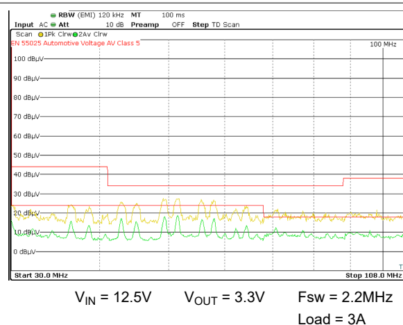
Figure 8-19. CISPR 25 Class 5 Conducted EMI 30 MHz–108MHz Yellow: Peak Detect, Green: Average Detect
