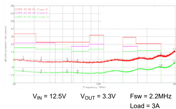
Figure 8-21. CISPR 25 Class 5 Radiated EMI, Biconical Antenna, Horizontal Polarization, 30MHz - 300MHz Red: Peak Detect, Green: Average Detect
