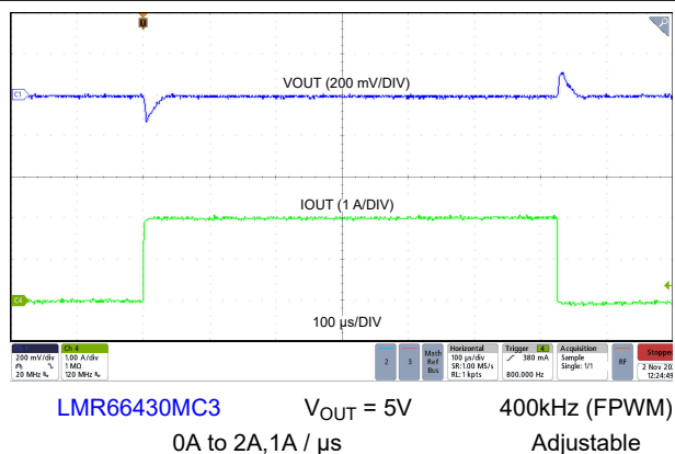
Figure 8-31. Load Transient
