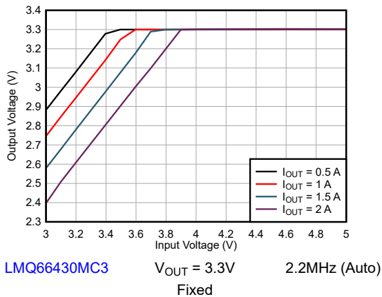
Figure 8-6. Dropout
