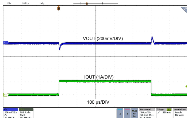
Figure 8-10. Load Transient
