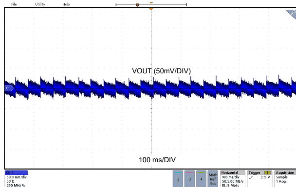
Figure 8-13. Load Transient
