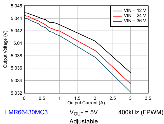
Figure 8-28. Line and Load Regulation
