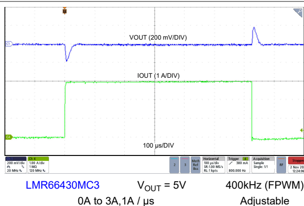
Figure 8-30. Load Transient
