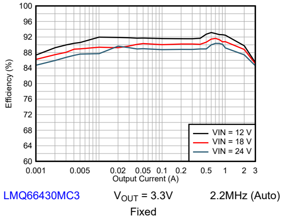
Figure 8-4. Efficiency
