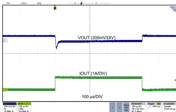
Figure 8-11. Load Transient
