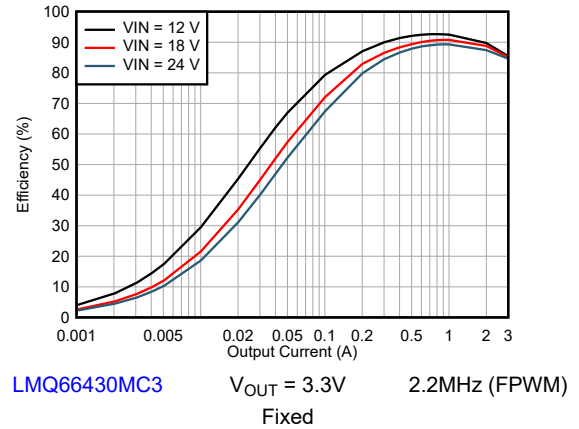
Figure 8-5. Efficiency
