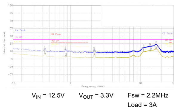
Figure 8-20. CISPR 25 Class 5 Radiated EMI, Rod Antenna, 150kHz–30MHz Blue: Peak Detect, Yellow: Average Detect
