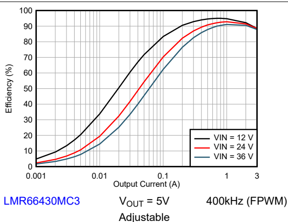
Figure 8-27. Efficiency
