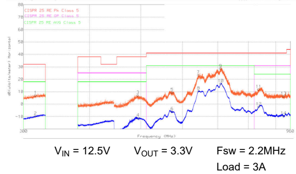
Figure 8-23. CISPR 25 Class 5 Radiated EMI, Log Antenna, Horizontal Polarization, 300MHz - 960MHz Orange: Peak Detect, Blue: Average Detect
