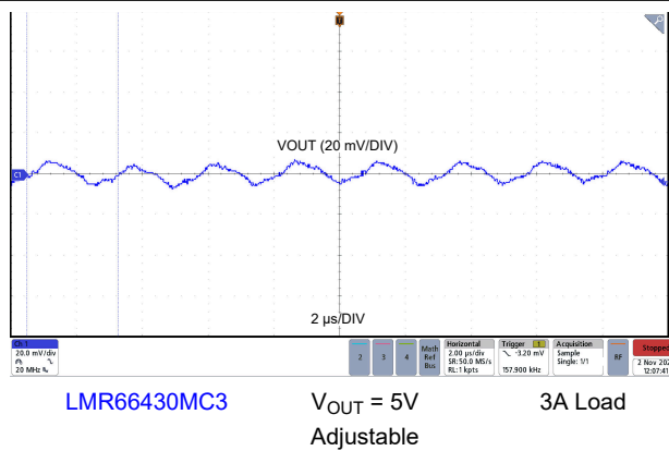
Figure 8-32. Output Voltage Ripple
