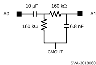
Figure 8. Typical Bandpass Filter
