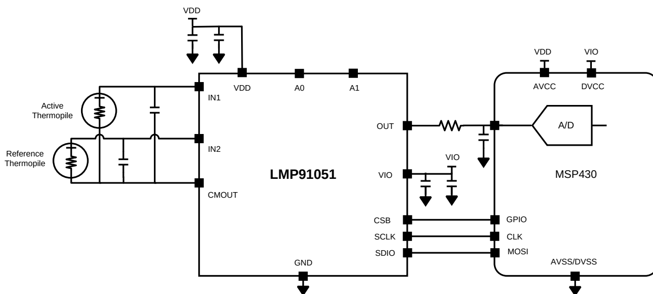
Typical NDIR Sensing Application Circuit
