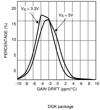
Figure 5-56. Gain Error Distribution at V_S = 5V LMP8603-Q1
