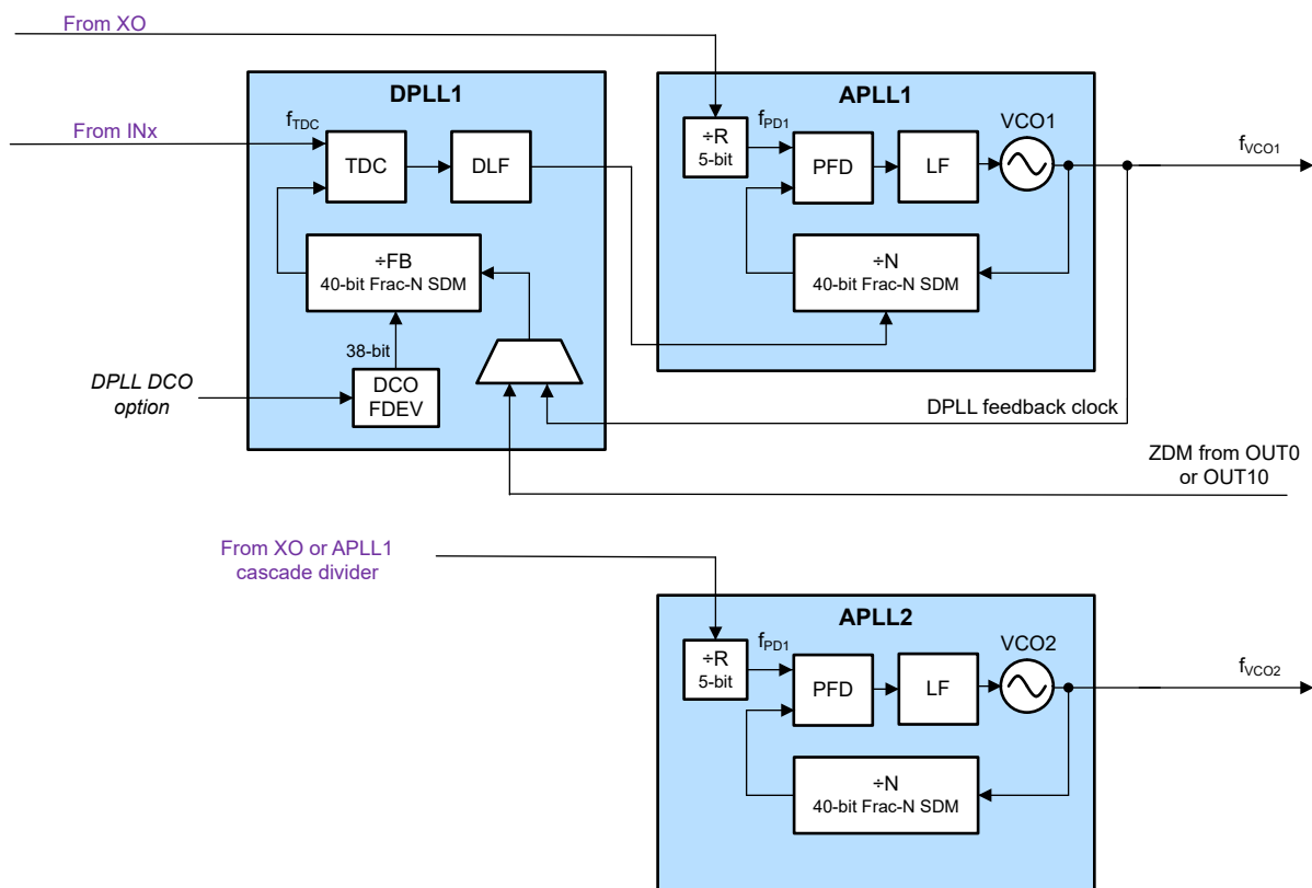
Figure 8-3. DPLL Operation
