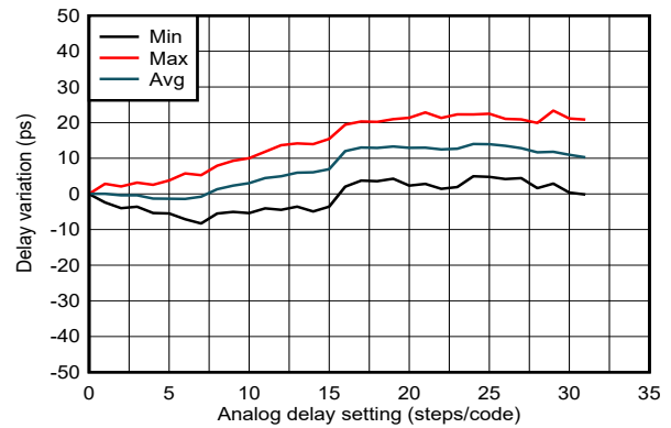
Figure 6-21. SYSREF/1PPS Delay Linearity vs. Analog Delay Code 4
