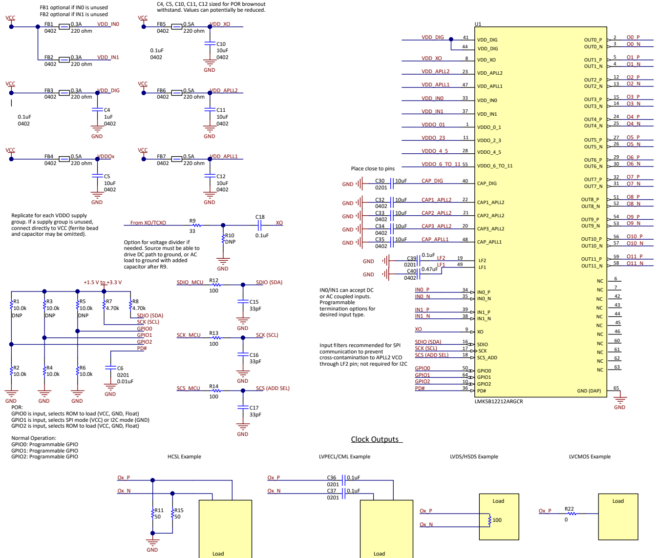
Figure 9-4. Reference Schematic Example
