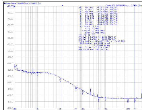
Figure 6-9. 156.25MHz HSDS Output From BAW APLL
