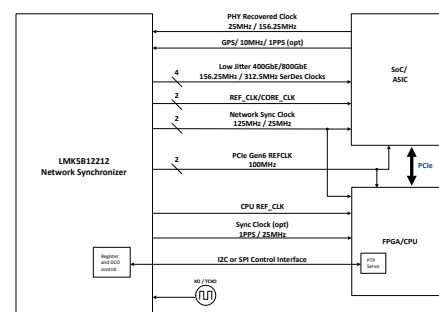
LMK5B12212 Typical System Block Diagram
