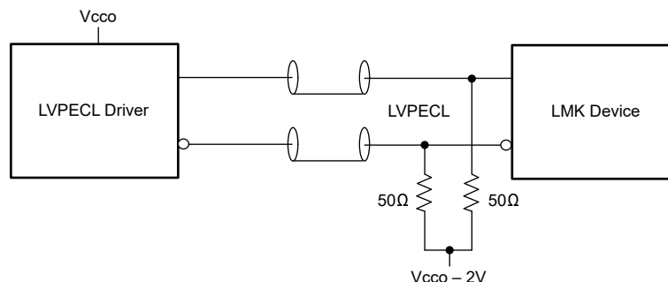
Figure 8-9. DC-Coupled LVPECL to Reference (INx)
