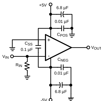
Figure 23. Recommended Inverting Gain Circuit, Gain = -1
