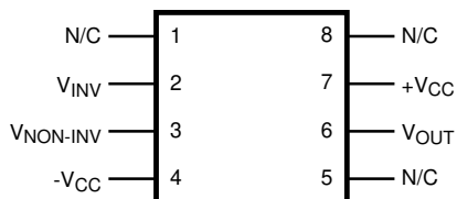
NAB Package, 8-Pin CDIP (Top View)
