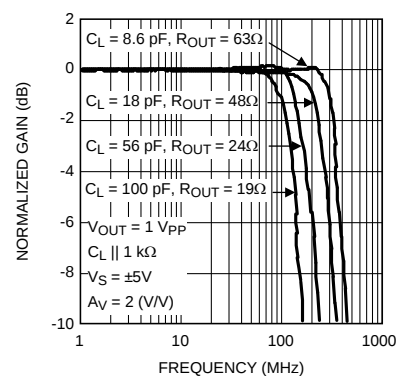
Figure 32. Decoupling Capacitive Loads
