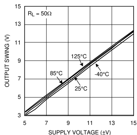
Figure 5-40. Positive Output Swing vs. Supply Voltage
