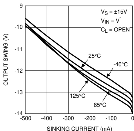
Figure 5-37. Negative Output Swing vs. Sinking Current
