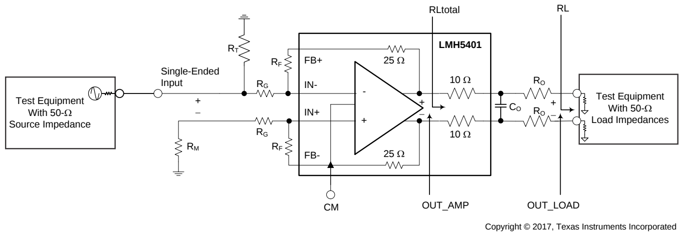
Figure 56. Test Schematic: Capacitive Load, G_V = 7 \text{ V/V}
