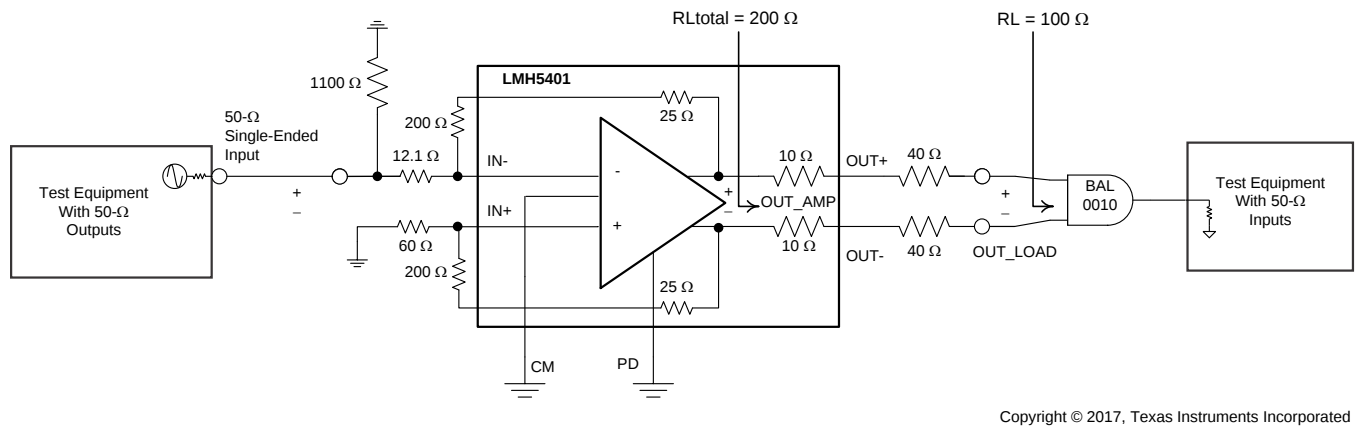
Figure 57. Test Schematic for Noise Figure and Single-Ended Harmonic Distortion, G_V = 7 \text{ V/V}
