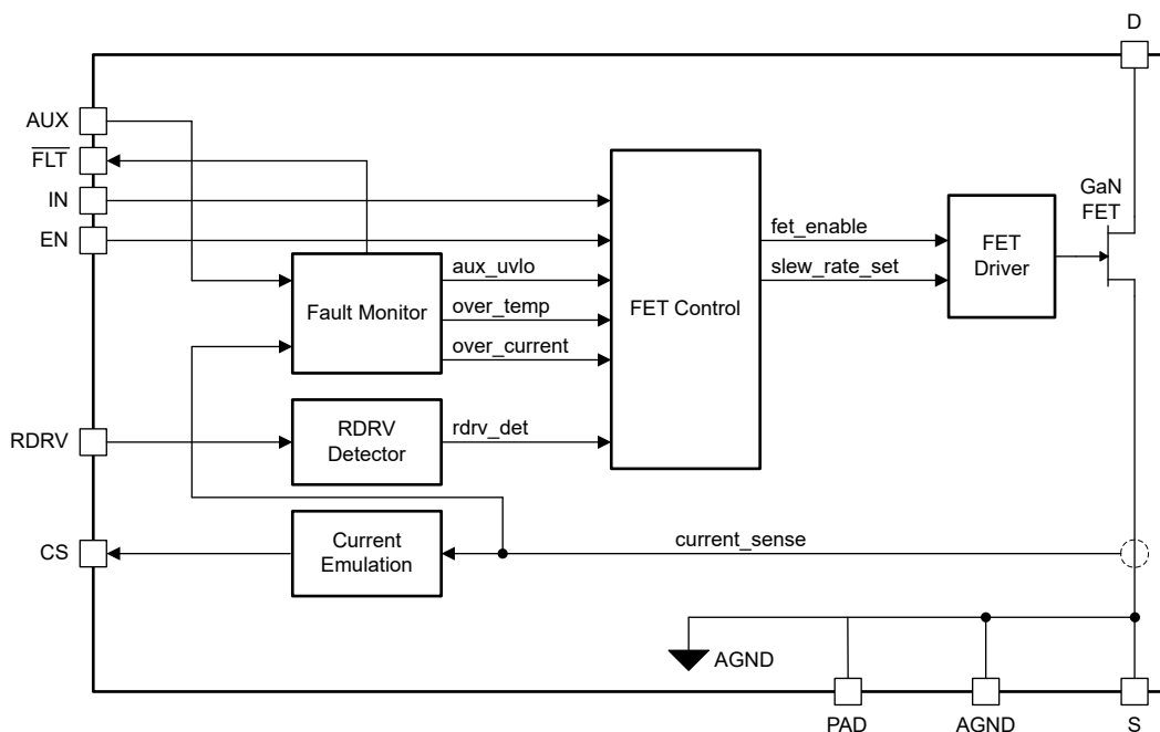
Figure 7-1. Functional Block Diagram
