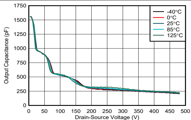
Figure 5-8. Output Capacitance vs Drain-Source Voltage
