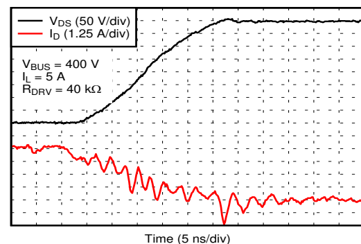
Figure 8-6. Turn-Off Waveform in Application Example
