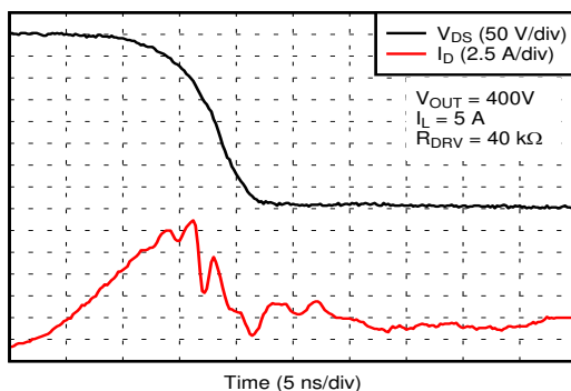
Figure 8-5. Turn-On Waveform in Application Example
