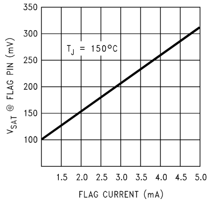
Figure 9-1. V_{SAT} vs Flag Current
