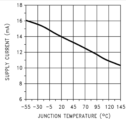
Figure 9-6. Supply Current vs Temperature ( V_S = 42V )
