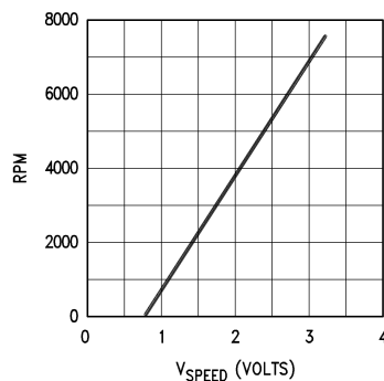
Figure 11-11. Motor Speed vs Control Voltage
