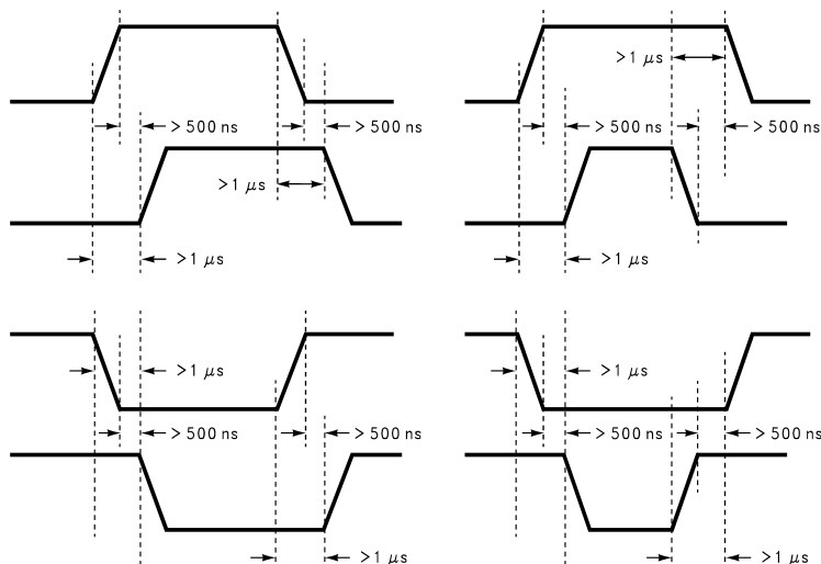
Figure 11-3. Transitions in Brake, Direction, or PWM Must Be Separated By At Least 1 μsec
