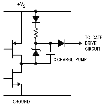
Figure 11-4. Internal Charge Pump Circuitry
