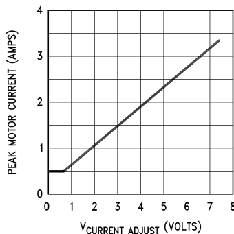
Figure 11-9. Peak Motor Current vs Adjustment Voltage
