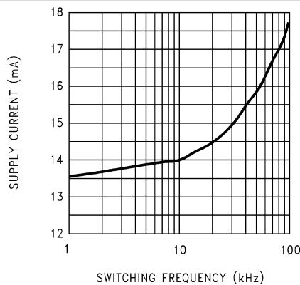
Figure 9-5. Supply Current vs Frequency ( V_S = 42V )
