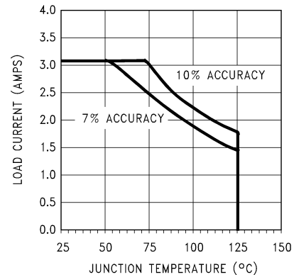
Figure 9-8. Current Sense Operating Region
