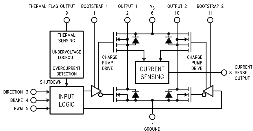
Figure 4-1. Functional Block Diagram of LMD18200
