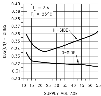
Figure 9-3. R_{DS(On)} vs Supply Voltage
