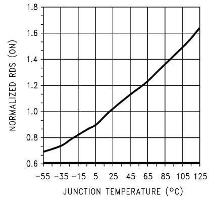
Figure 9-2. R_{DS(On)} vs Temperature
