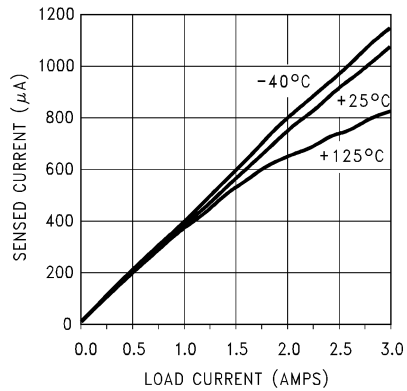
Figure 9-7. Current Sense Output vs Load Current
