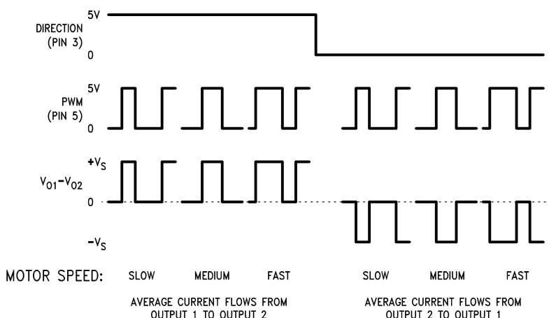
Figure 11-2. Sign/Magnitude PWM Control
