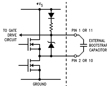
Figure 11-5. Bootstrap Circuitry
