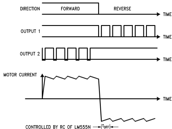
Figure 11-7. Switching Waveforms
