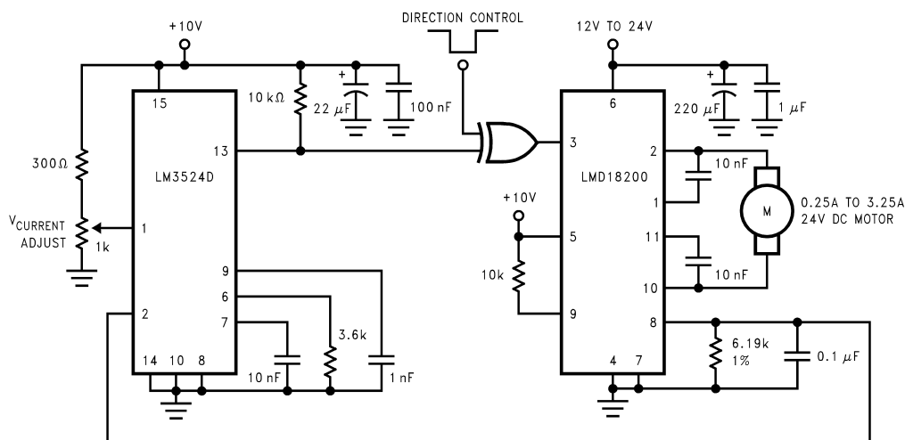
Figure 11-8. Locked Anti-Phase Control Regulates Torque
