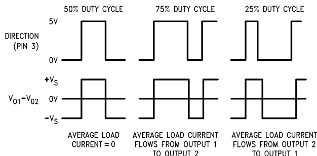
Figure 11-1. Locked Anti-Phase PWM Control
