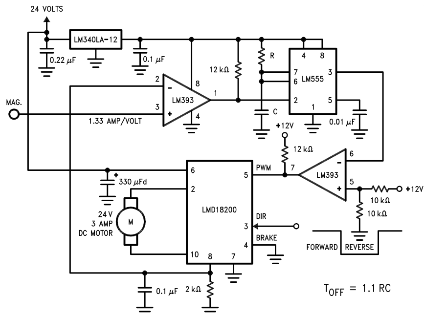
Figure 11-6. Fixed Off-Time Control
