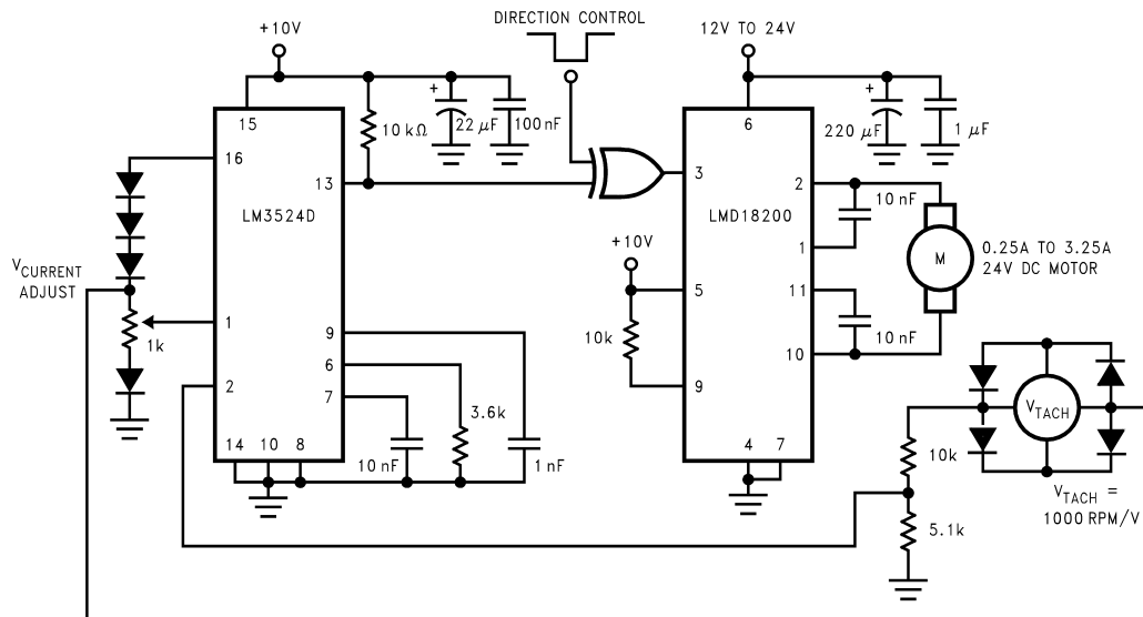
Figure 11-10. Regulate Velocity with Tachometer Feedback
