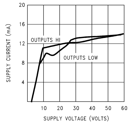
Figure 9-4. Supply Current vs Supply Voltage
