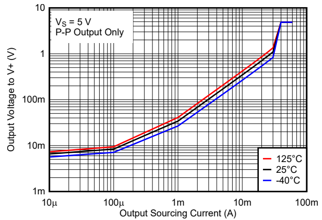
Figure 4-4. Output Voltage vs. Output Sourcing Current, 5V
