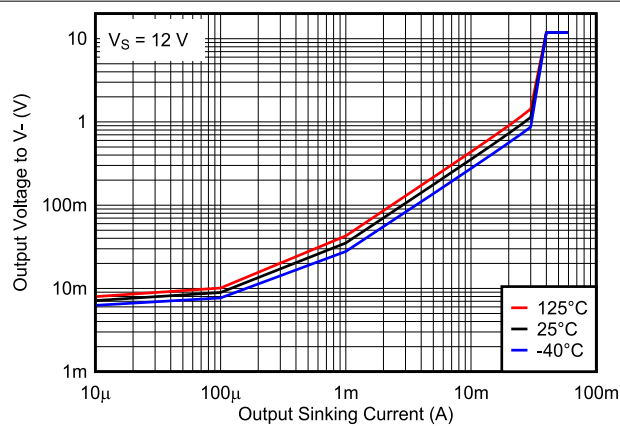
Figure 4-5. Output Voltage vs. Output Sinking Current, 12V
