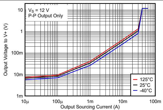
Figure 4-6. Output Voltage vs. Output Sourcing Current, 12V
