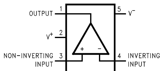
5-Pin SOT23-5 Top View
