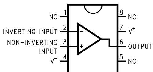
8-Pin SOIC-8 Top View
