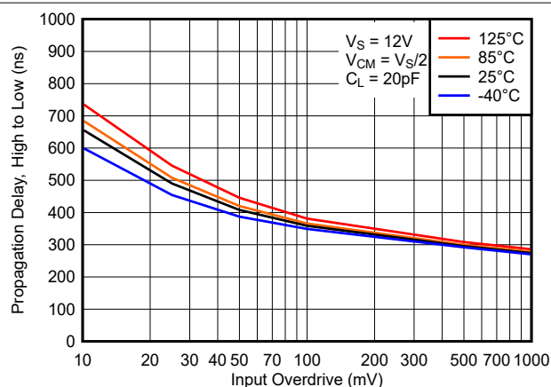
Figure 5-6. Propagation Delay, High to Low, 12V
