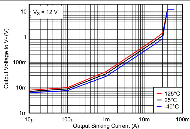
Figure 5-4. Output Voltage vs. Output Sinking Current, 12V
