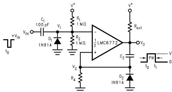
Figure 6-5. One-Shot Multivibrator
