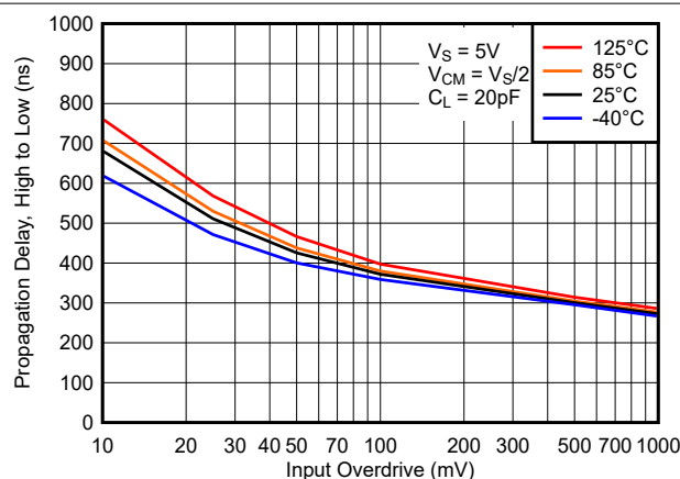
Figure 5-5. Propagation Delay, High to Low, 5V
