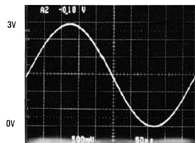
Rail-To-Rail Output
