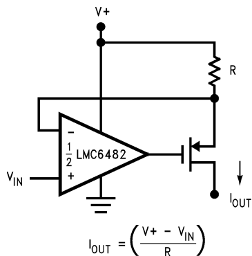
Figure 73. Large Compliance Range Current Source
