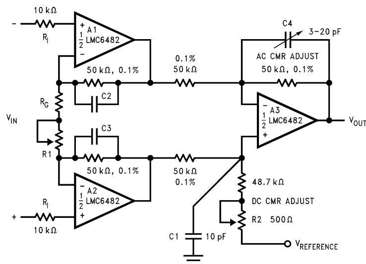
Figure 67. Low Power 3 Op-Amp Instrumentation Amplifier
