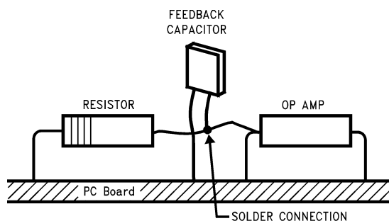
Figure 63. Air Wiring
