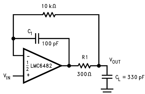
Figure 58. LMC6482 Noninverting Amplifier, Compensated to Handle a 330pF Capacitive Load
