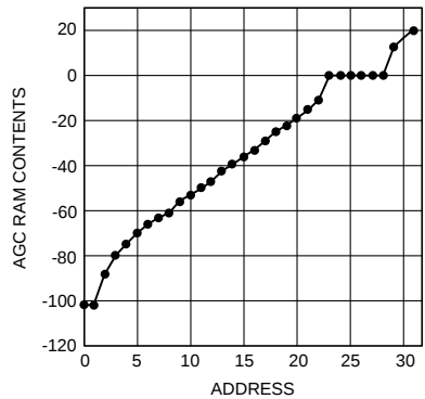
Figure 83. Example of programmed RAM contents
