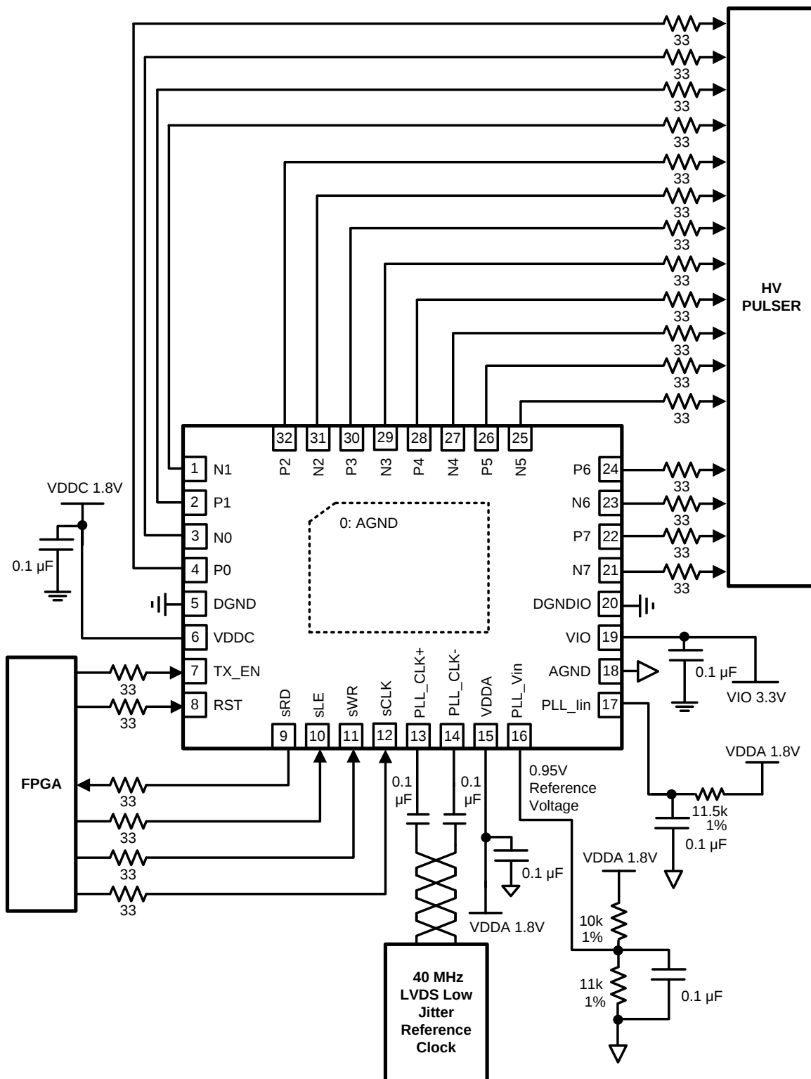
Figure 16. REFERENCE CIRCUIT
