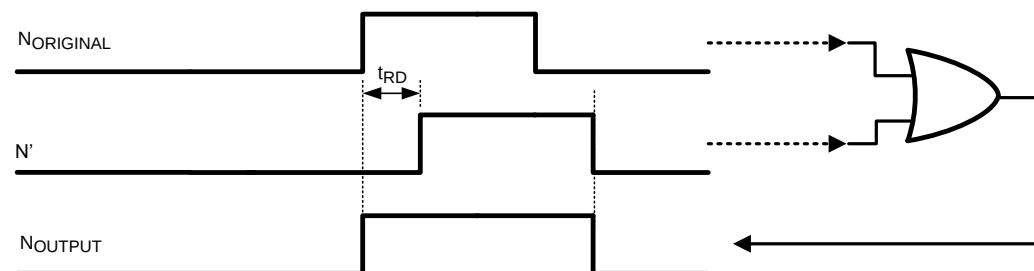
Figure 14. Pulse Width Adjustment (00h[21:20] = "10")
