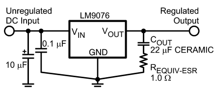
Figure 24. Using Low ESR Capacitors
