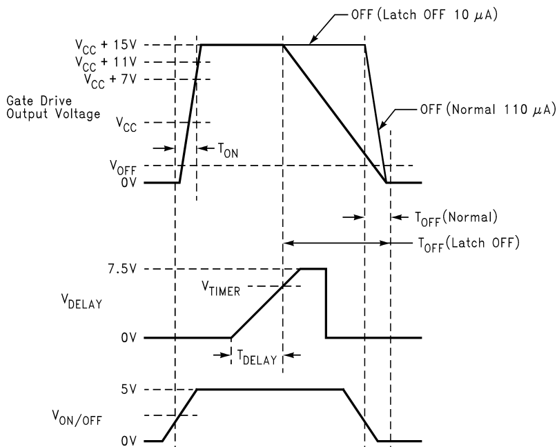
Figure 2. Timing Definitions
