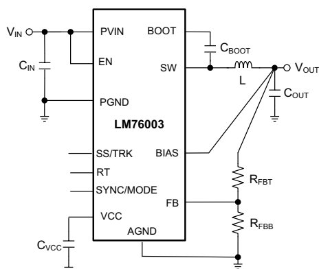
Simplified Schematic
