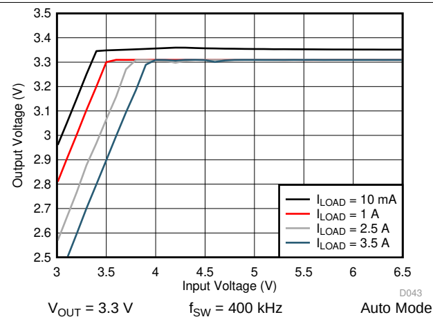
Figure 51. LM76003-Q1 Dropout Curve
