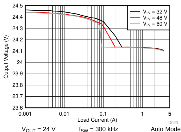
Figure 47. LM76003-Q1 Load and Line Regulation
