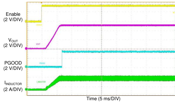
Figure 67. LM76003-Q1 Start-up Waveform
