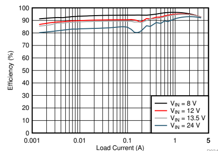
Efficiency vs Output Current ( V_{\text{OUT}} = 5 \text{ V} , f_{\text{SW}} = 400 \text{ kHz} , Auto Mode)
