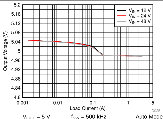
Figure 49. LM76002-Q1 Load and Line Regulation
