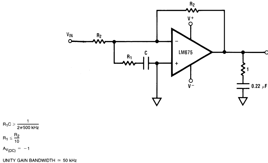
Figure 13. Inverting Unity Gain Operation
