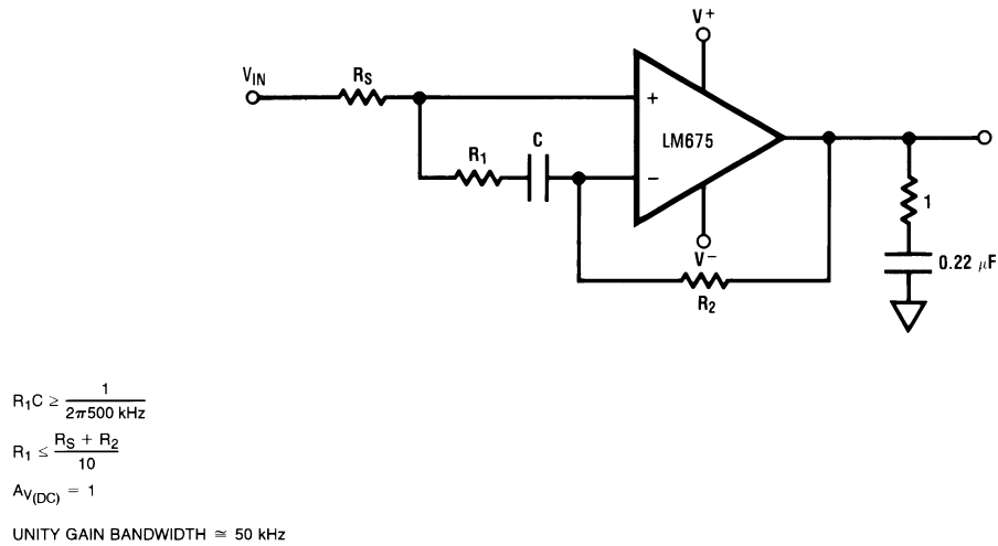
Figure 12. Non-Inverting Unity Gain Operation
