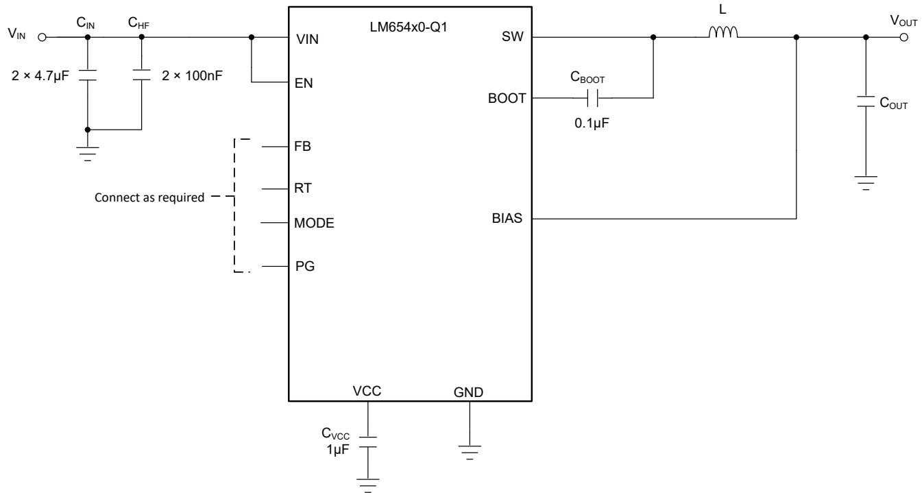
Figure 8-2. Example Application Circuit for Fixed Output Voltage Mode With LM654X0-Q1
