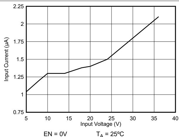
Figure 6-1. Shutdown Current
