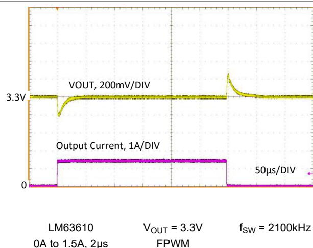
Figure 8-14. Load Transient
