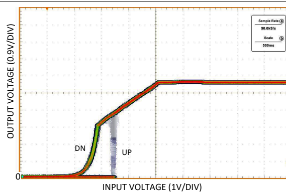
Figure 6-2. UVLO Thresholds
