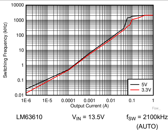
Figure 8-11. Switching Frequency versus Output Current
