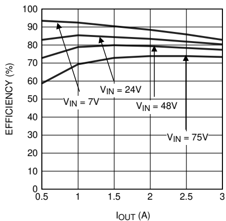
Figure 5-9. Demoboard Efficiency vs I_{OUT} and V_{IN}
