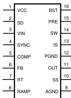
Figure 4-1. PWP Package 16-Pin HTSSOP (Top View)
