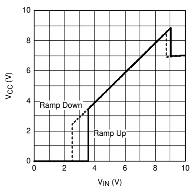
Figure 5-5. V_{CC} vs V_{IN} R_I = 7\text{k}\Omega
