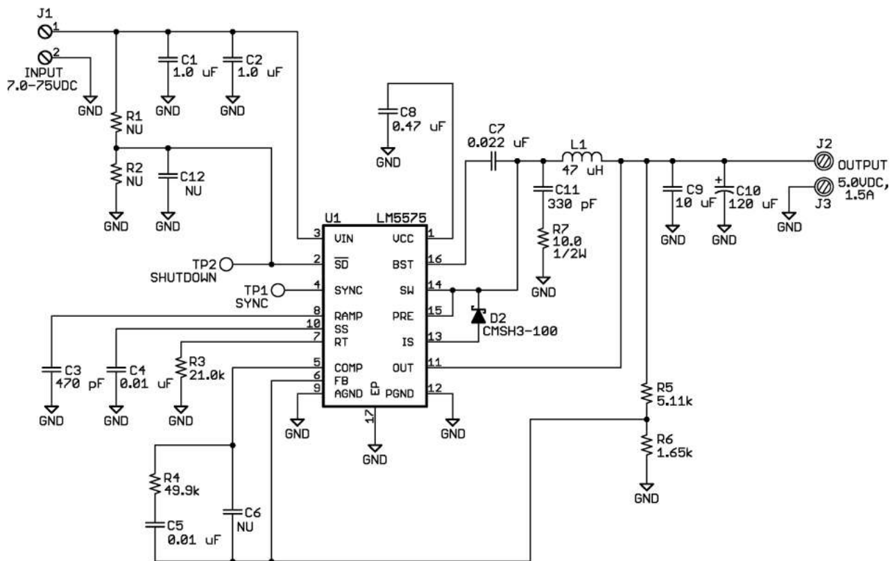
Figure 7-3. Schematic Diagram
