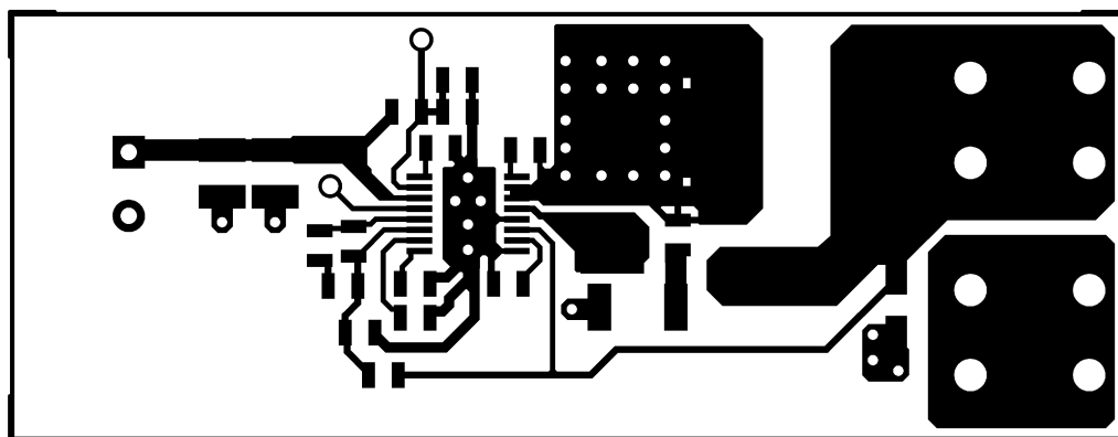
Figure 7-12. Component Side
