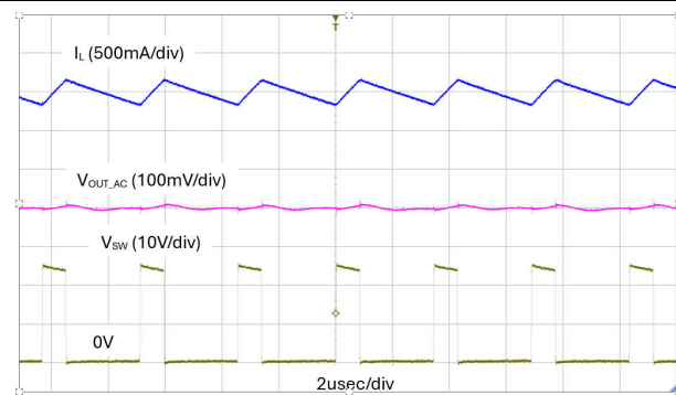
Figure 7-10. Steady State Waveform ( V_{IN} = 24V , V_{OUT}=5V , I_{OUT} = 1.5A )
