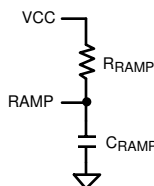
Figure 6-6. R to V for V > 7.5V_{RAMP} CC OUT
