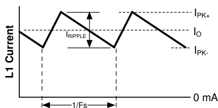
Figure 7-4. Inductor Current Waveform
