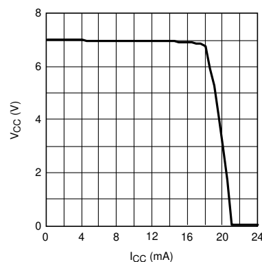
Figure 5-4. V_{CC} vs I_{CC} V_{IN} = 12\text{V}
