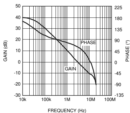
Figure 5-6. Error Amplifier Gain/Phase A_{vcl} = 101
