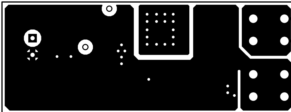
Figure 7-13. Solder Side
