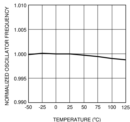
Figure 5-2. Oscillator Frequency VS Temperature F_{osc} = 200\text{kHz}
