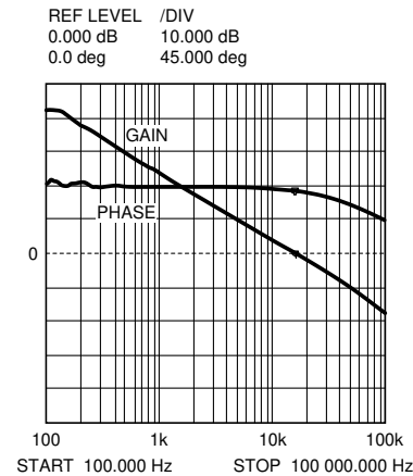
Figure 7-9. Overall Loop Gain and Phase
