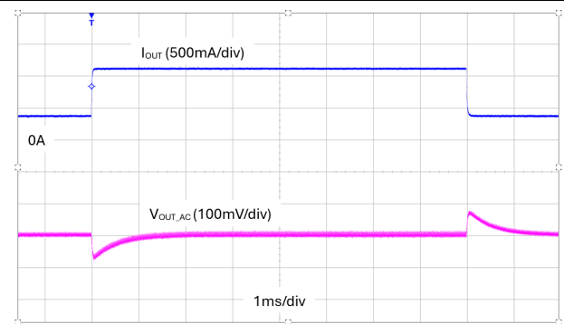
Figure 7-11. Load Transient Response ( V_{IN} = 24V , V_{OUT}=5V , I_{OUT} = 400mA to 1.2A )
