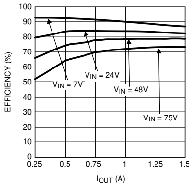
Figure 7-8. Demoboard Efficiency Vs I_{OUT} and V_{IN}
