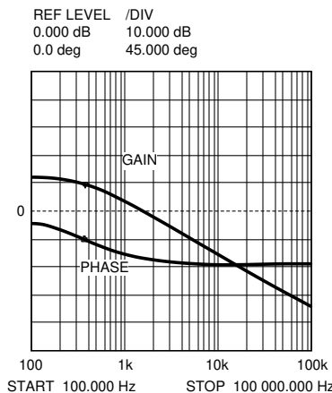
Figure 7-5. Gain and Phase of Modulator R = 5Ω and C = 130 μF
