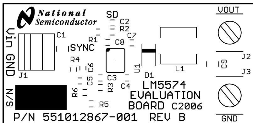
Figure 7-14. Silkscreen
