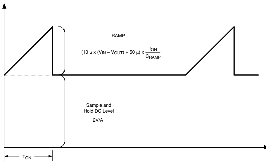
Figure 6-5. Composition of Current Sense Signal
