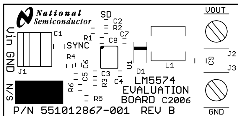
Figure 7-14. Silkscreen
